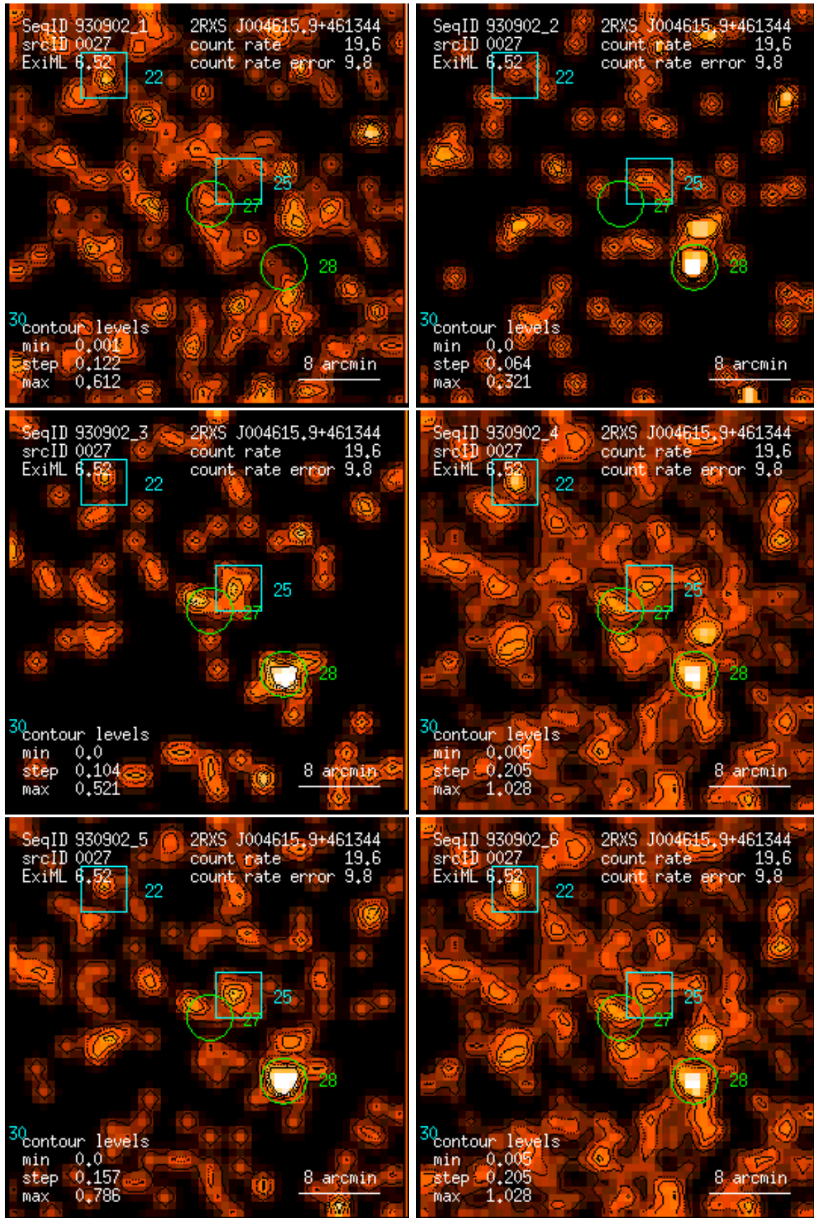
Figure 27: RASS 930902: detection 0027: band rate images, Gaussian filter: (1) PSPC channels 11 – 41, (2) 52 – 90, (3) 91 – 201, (4) 11 – 235, (5) 52 – 201, (6) 11 – 201. Broad band rates in counts/ks. Band rate contour levels in counts/ks/arcmin 2 .
