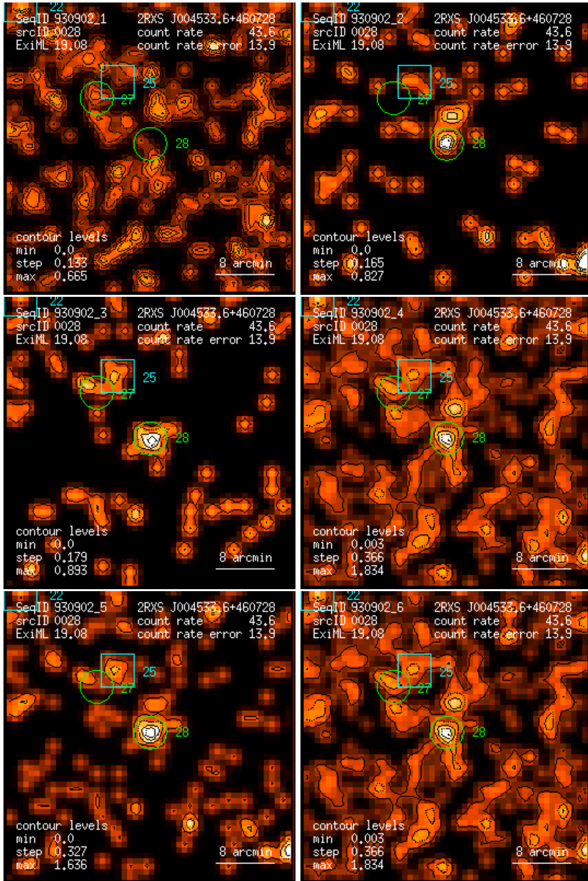
Figure 28: RASS 930902: detection 0028: band rate images, Gaussian filter: (1) PSPC channels 11 – 41, (2) 52 – 90, (3) 91 – 201, (4) 11 – 235, (5) 52 – 201, (6) 11 – 201. Broad band rates in counts/ks. Band rate contour levels in counts/ks/arcmin 2 .
