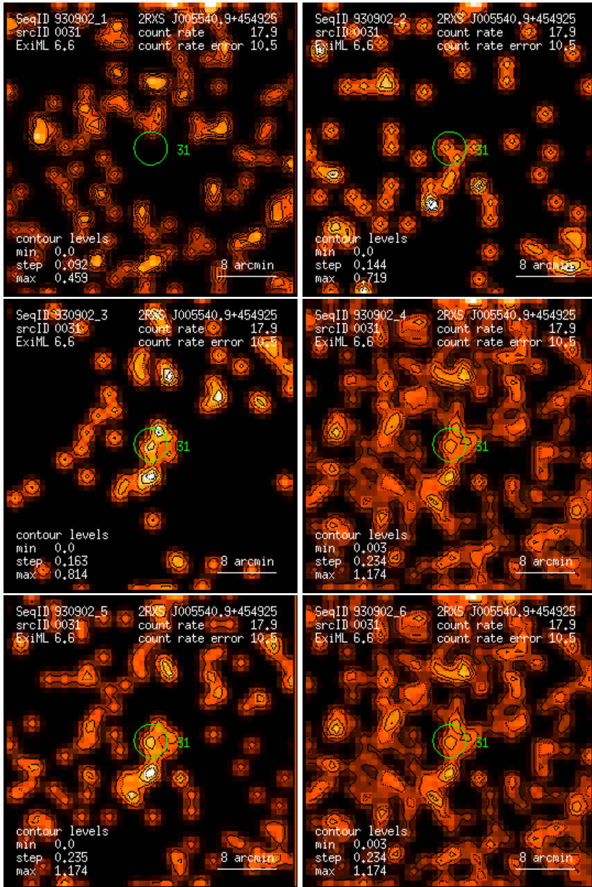
Figure 31: RASS 930902: detection 0031: band rate images, Gaussian filter: (1) PSPC channels 11 – 41, (2) 52 – 90, (3) 91 – 201, (4) 11 – 235, (5) 52 – 201, (6) 11 – 201. Broad band rates in counts/ks. Band rate contour levels in counts/ks/arcmin 2 .
