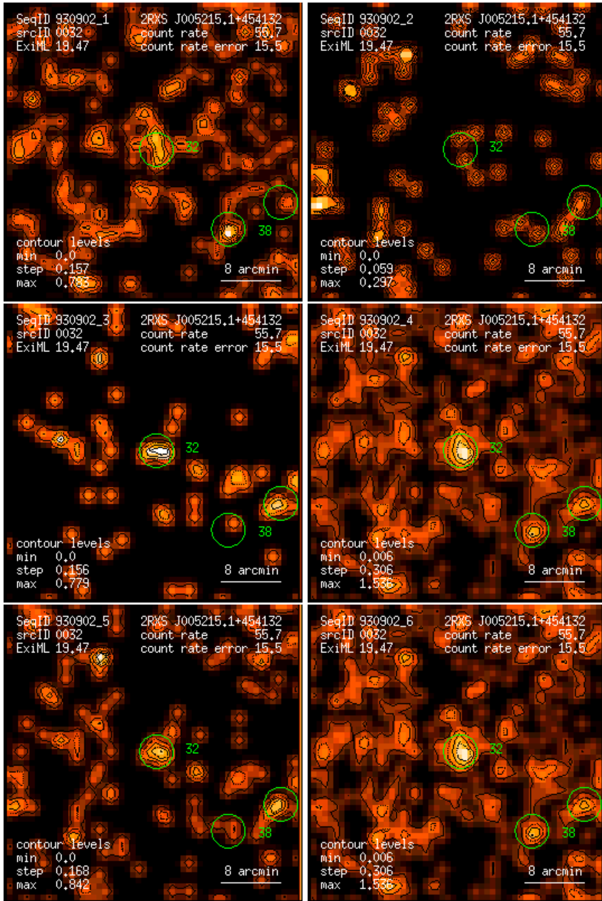
Figure 32: RASS 930902: detection 0032: band rate images, Gaussian filter: (1) PSPC channels 11 – 41, (2) 52 – 90, (3) 91 – 201, (4) 11 – 235, (5) 52 – 201, (6) 11 – 201. Broad band rates in counts/ks. Band rate contour levels in counts/ks/arcmin 2 .
