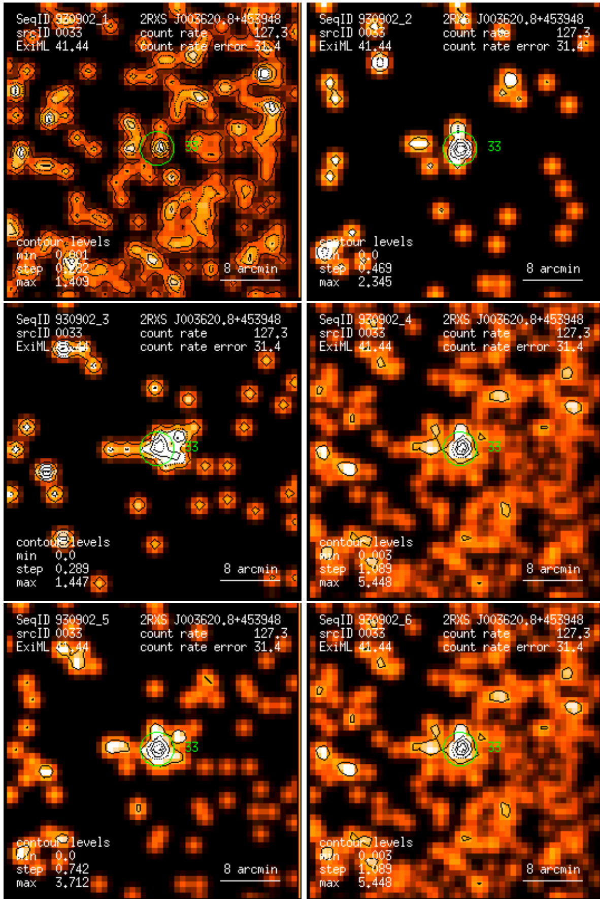
Figure 33: RASS 930902: detection 0033: band rate images, Gaussian filter: (1) PSPC channels 11 – 41, (2) 52 – 90, (3) 91 – 201, (4) 11 – 235, (5) 52 – 201, (6) 11 – 201. Broad band rates in counts/ks. Band rate contour levels in counts/ks/arcmin 2 .
