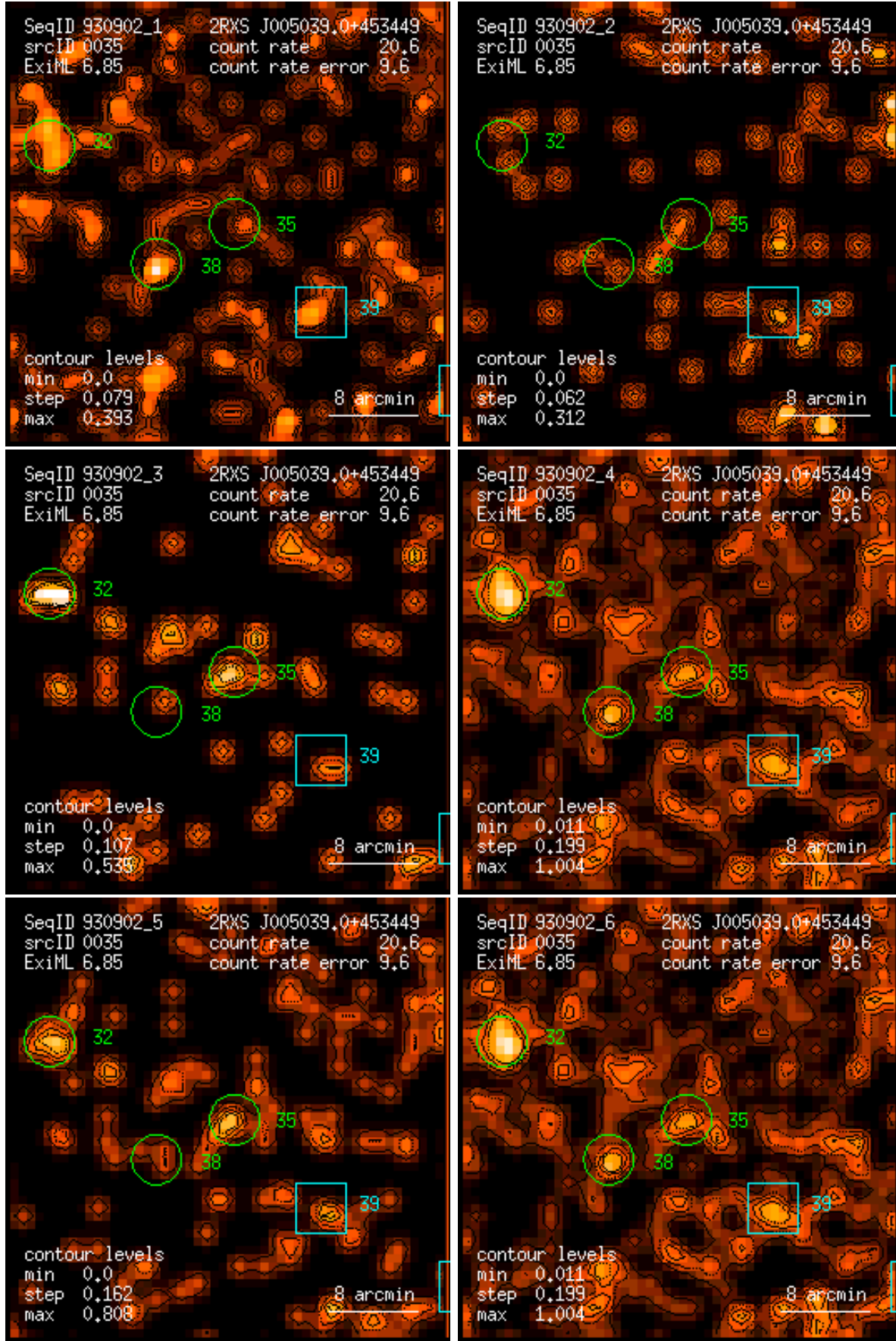
Figure 35: RASS 930902: detection 0035: band rate images, Gaussian filter: (1) PSPC channels 11 – 41, (2) 52 – 90, (3) 91 – 201, (4) 11 – 235, (5) 52 – 201, (6) 11 – 201. Broad band rates in counts/ks. Band rate contour levels in counts/ks/arcmin 2 .
