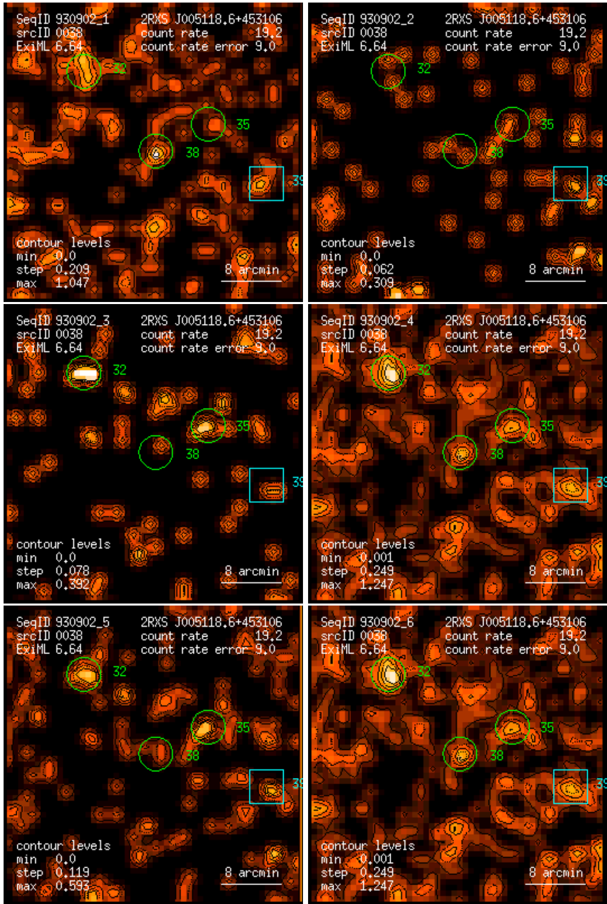
Figure 38: RASS 930902: detection 0038: band rate images, Gaussian filter: (1) PSPC channels 11 – 41, (2) 52 – 90, (3) 91 – 201, (4) 11 – 235, (5) 52 – 201, (6) 11 – 201. Broad band rates in counts/ks. Band rate contour levels in counts/ks/arcmin 2 .
