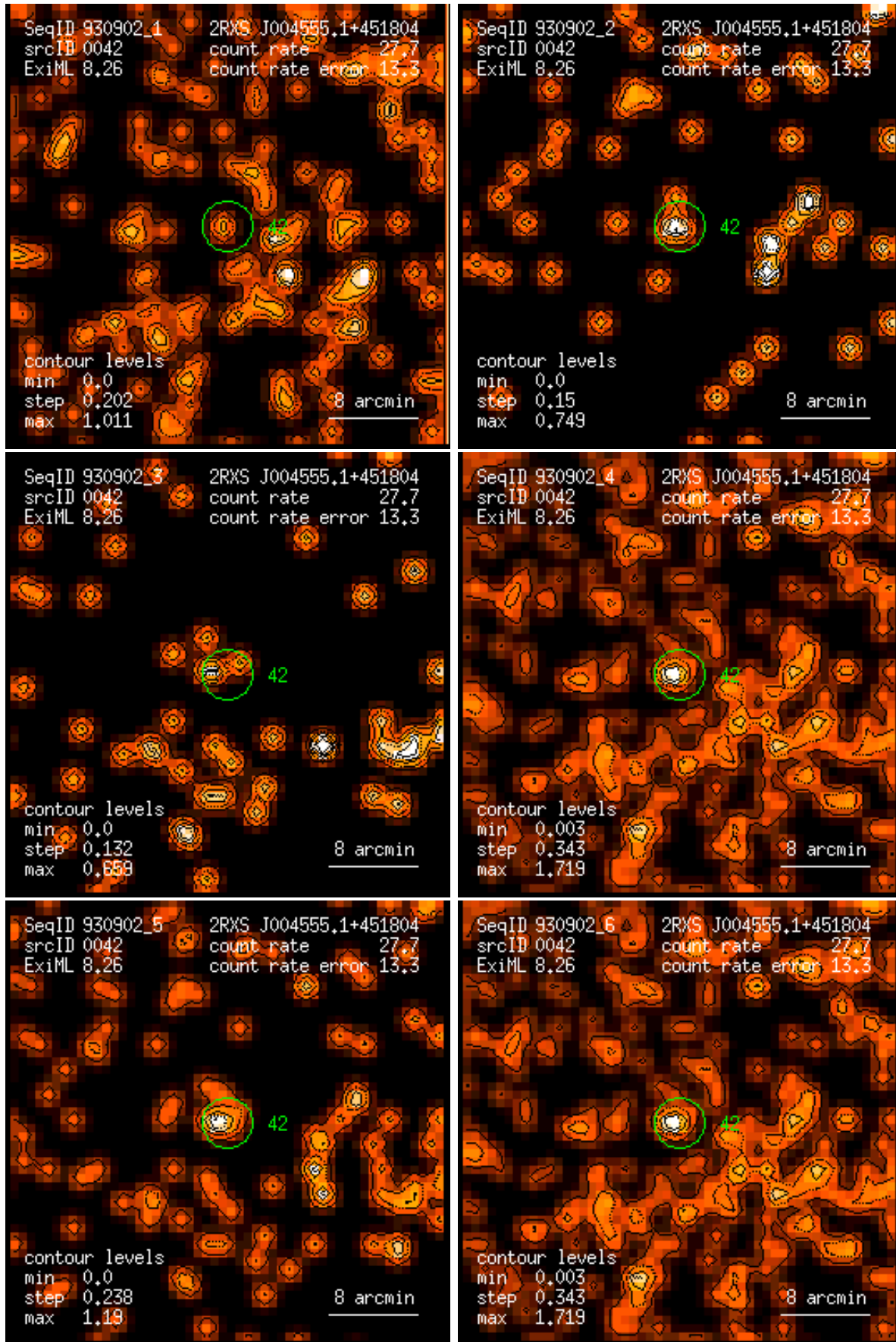
Figure 42: RASS 930902: detection 0042: band rate images, Gaussian filter: (1) PSPC channels 11 – 41, (2) 52 – 90, (3) 91 – 201, (4) 11 – 235, (5) 52 – 201, (6) 11 – 201. Broad band rates in counts/ks. Band rate contour levels in counts/ks/arcmin 2 .
