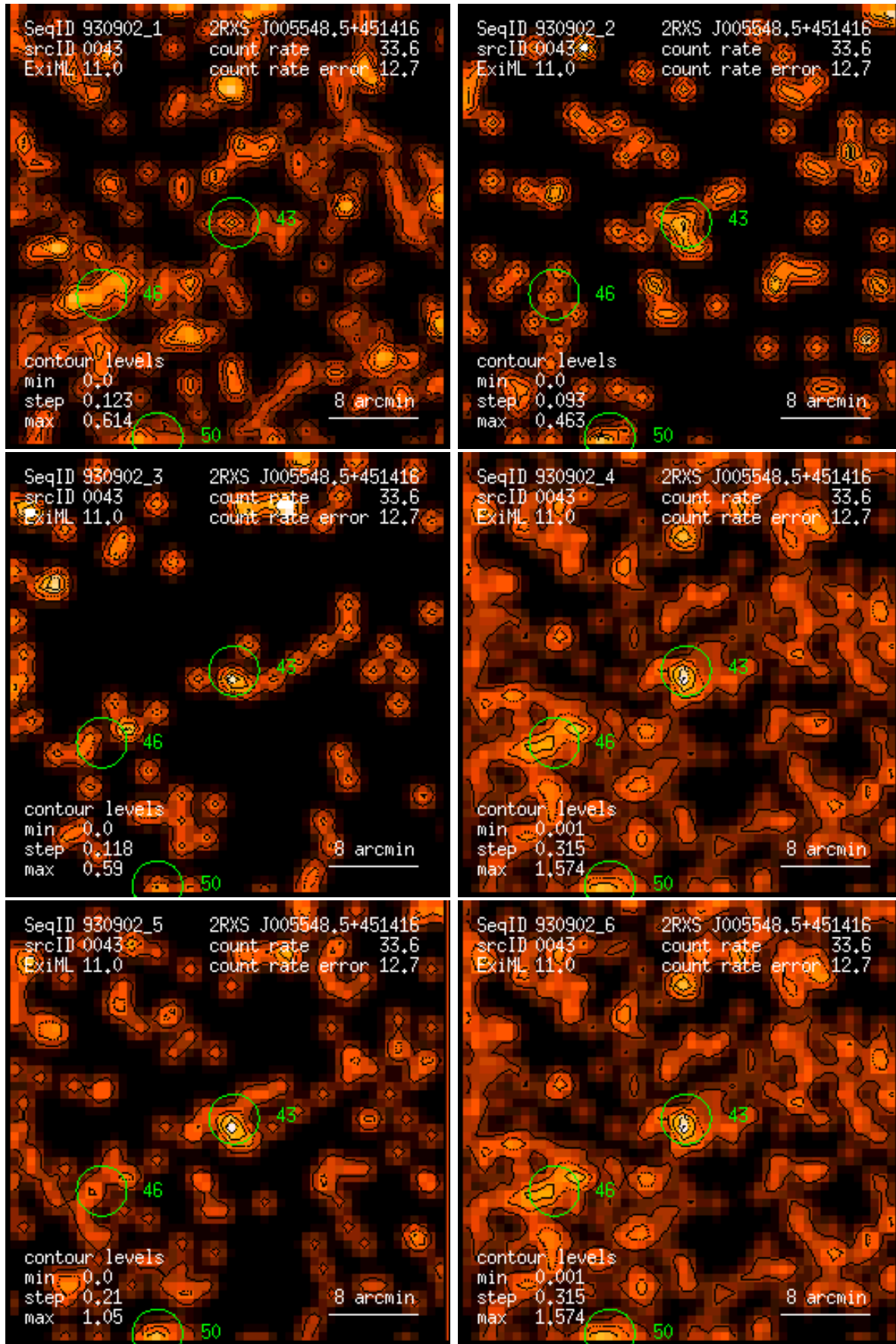
Figure 43: RASS 930902: detection 0043: band rate images, Gaussian filter: (1) PSPC channels 11 – 41, (2) 52 – 90, (3) 91 – 201, (4) 11 – 235, (5) 52 – 201, (6) 11 – 201. Broad band rates in counts/ks. Band rate contour levels in counts/ks/arcmin 2 .
