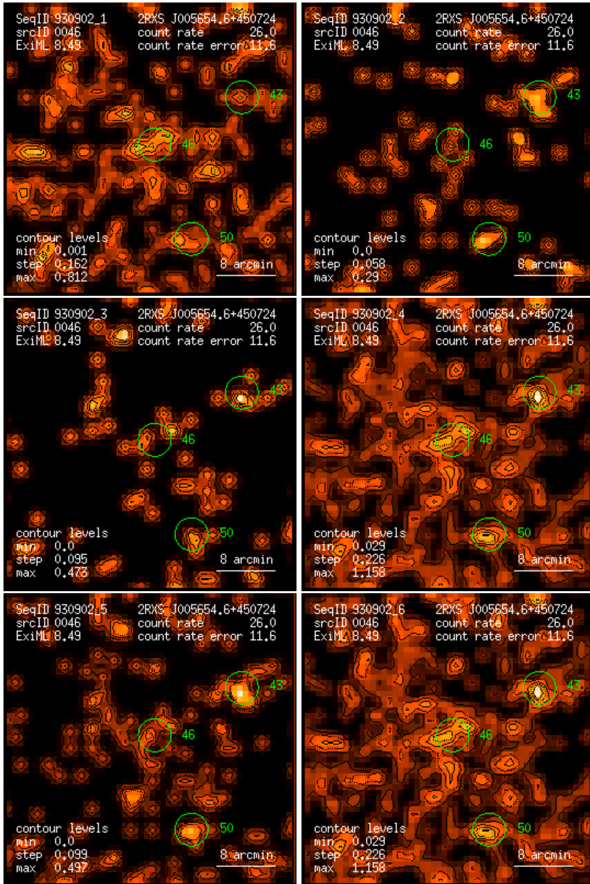
Figure 46: RASS 930902: detection 0046: band rate images, Gaussian filter: (1) PSPC channels 11 – 41, (2) 52 – 90, (3) 91 – 201, (4) 11 – 235, (5) 52 – 201, (6) 11 – 201. Broad band rates in counts/ks. Band rate contour levels in counts/ks/arcmin 2 .
