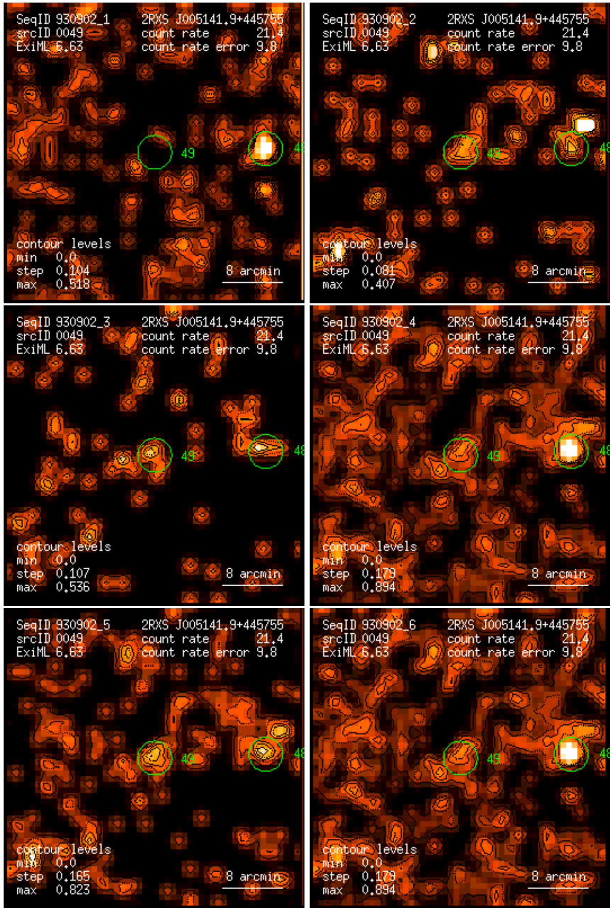
Figure 49: RASS 930902: detection 0049: band rate images, Gaussian filter: (1) PSPC channels 11 – 41, (2) 52 – 90, (3) 91 – 201, (4) 11 – 235, (5) 52 – 201, (6) 11 – 201. Broad band rates in counts/ks. Band rate contour levels in counts/ks/arcmin 2 .
