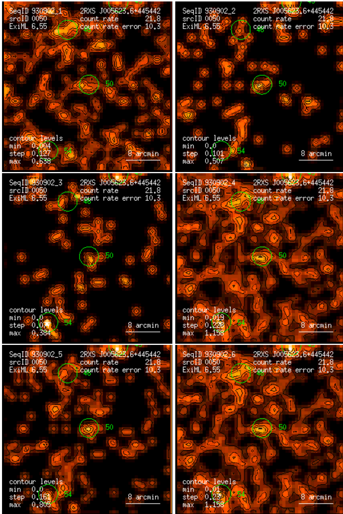
Figure 50: RASS 930902: detection 0050: band rate images, Gaussian filter: (1) PSPC channels 11 – 41, (2) 52 – 90, (3) 91 – 201, (4) 11 – 235, (5) 52 – 201, (6) 11 – 201. Broad band rates in counts/ks. Band rate contour levels in counts/ks/arcmin 2 .
