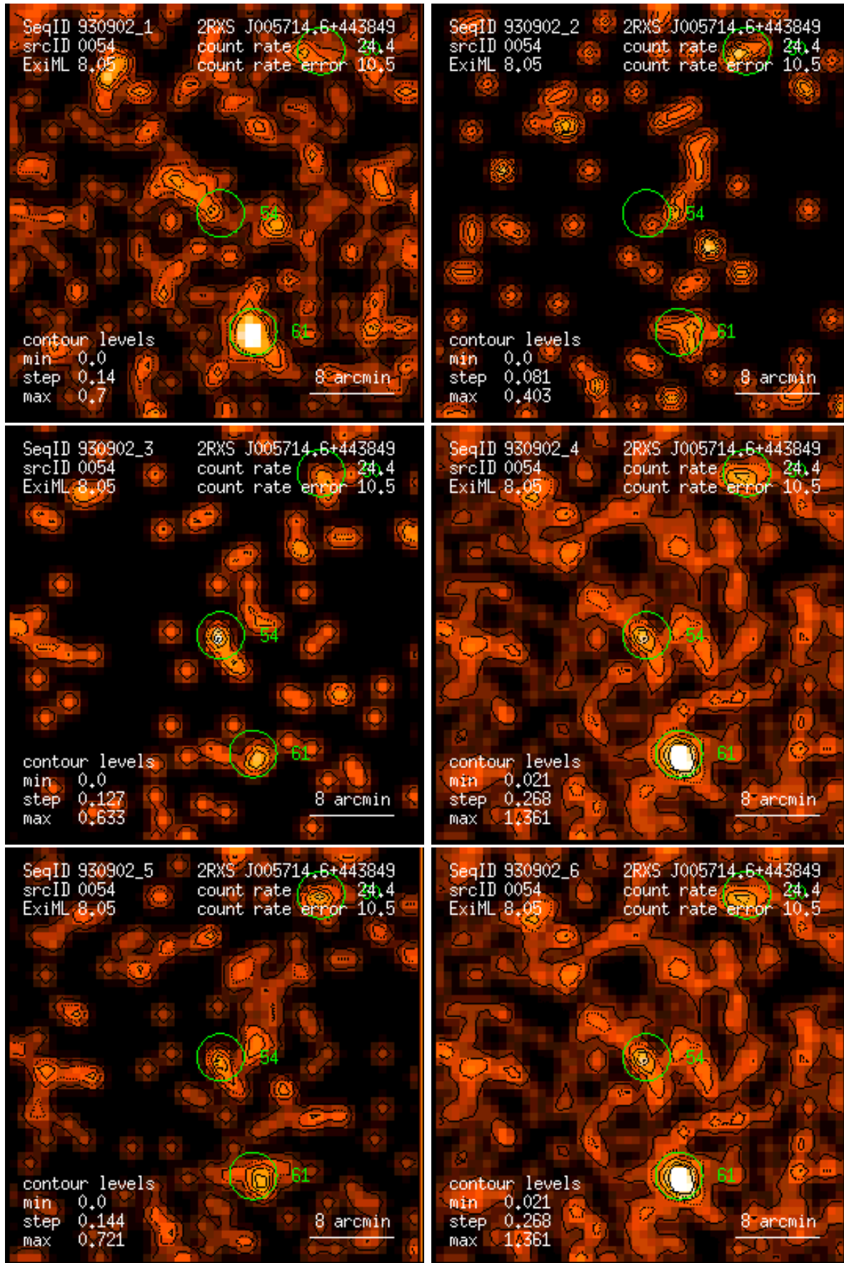
Figure 54: RASS 930902: detection 0054: band rate images, Gaussian filter: (1) PSPC channels 11 – 41, (2) 52 – 90, (3) 91 – 201, (4) 11 – 235, (5) 52 – 201, (6) 11 – 201. Broad band rates in counts/ks. Band rate contour levels in counts/ks/arcmin 2 .
