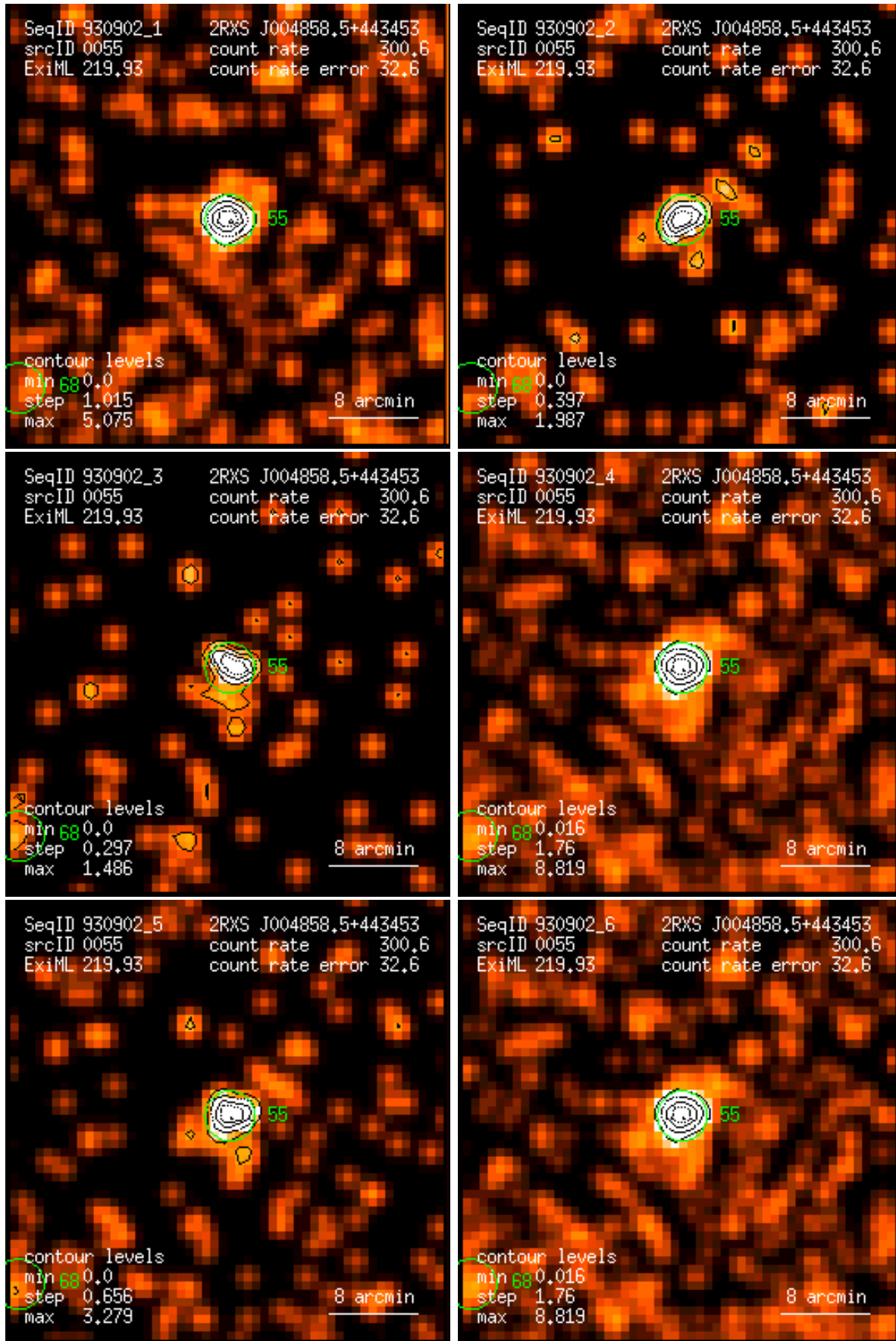
Figure 55: RASS 930902: detection 0055: band rate images, Gaussian filter: (1) PSPC channels 11 – 41, (2) 52 – 90, (3) 91 – 201, (4) 11 – 235, (5) 52 – 201, (6) 11 – 201. Broad band rates in counts/ks. Band rate contour levels in counts/ks/arcmin 2 .
