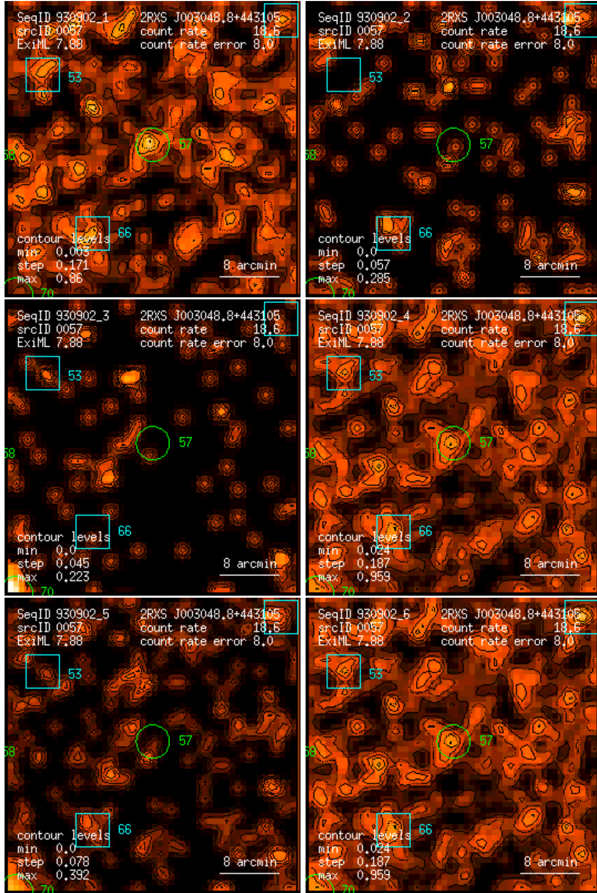
Figure 57: RASS 930902: detection 0057: band rate images, Gaussian filter: (1) PSPC channels 11 – 41, (2) 52 – 90, (3) 91 – 201, (4) 11 – 235, (5) 52 – 201, (6) 11 – 201. Broad band rates in counts/ks. Band rate contour levels in counts/ks/arcmin 2 .
