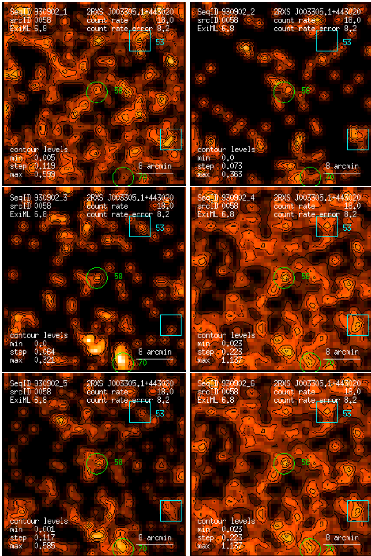
Figure 58: RASS 930902: detection 0058: band rate images, Gaussian filter: (1) PSPC channels 11 – 41, (2) 52 – 90, (3) 91 – 201, (4) 11 – 235, (5) 52 – 201, (6) 11 – 201. Broad band rates in counts/ks. Band rate contour levels in counts/ks/arcmin 2 .
