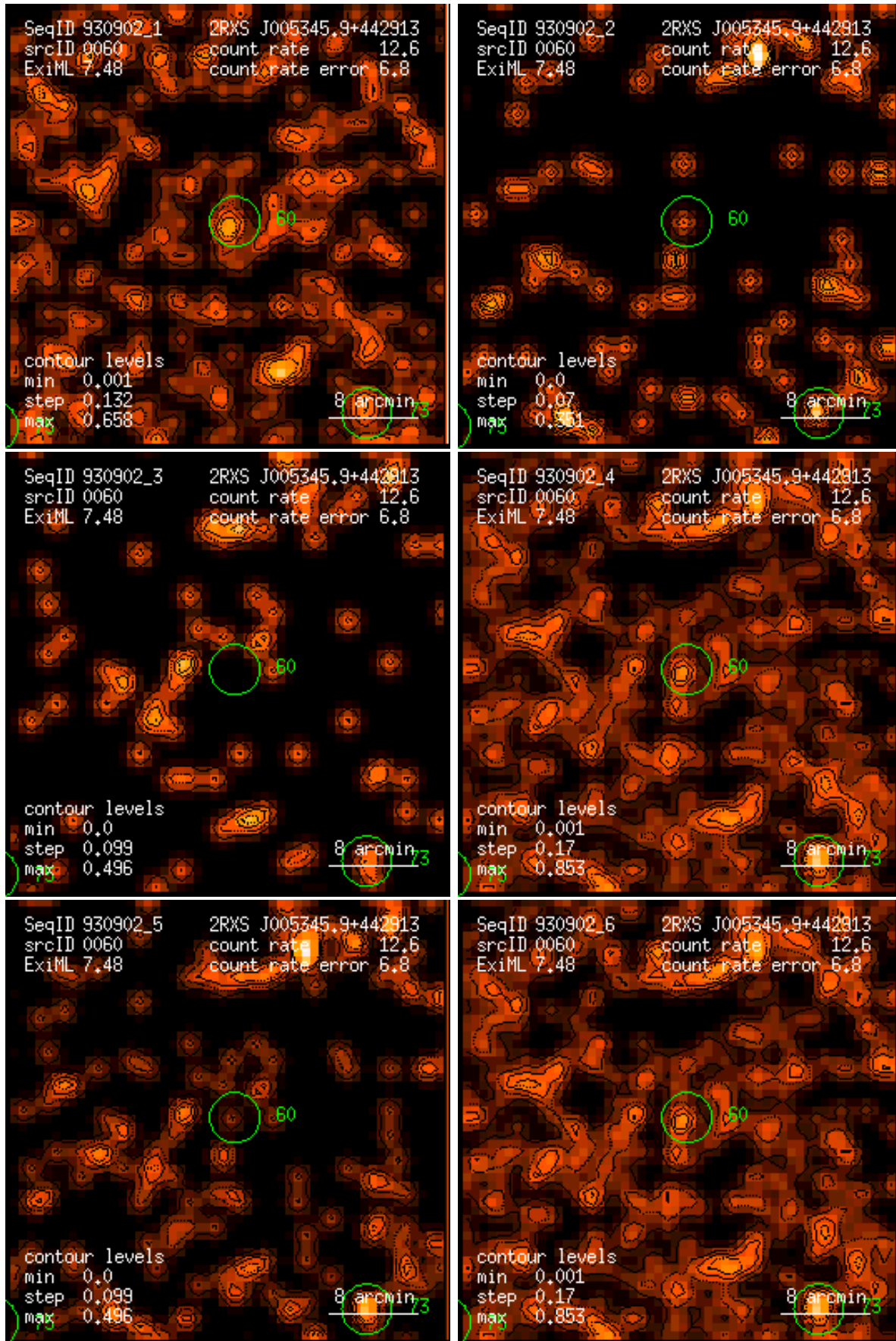
Figure 60: RASS 930902: detection 0060: band rate images, Gaussian filter: (1) PSPC channels 11 – 41, (2) 52 – 90, (3) 91 – 201, (4) 11 – 235, (5) 52 – 201, (6) 11 – 201. Broad band rates in counts/ks. Band rate contour levels in counts/ks/arcmin 2 .
