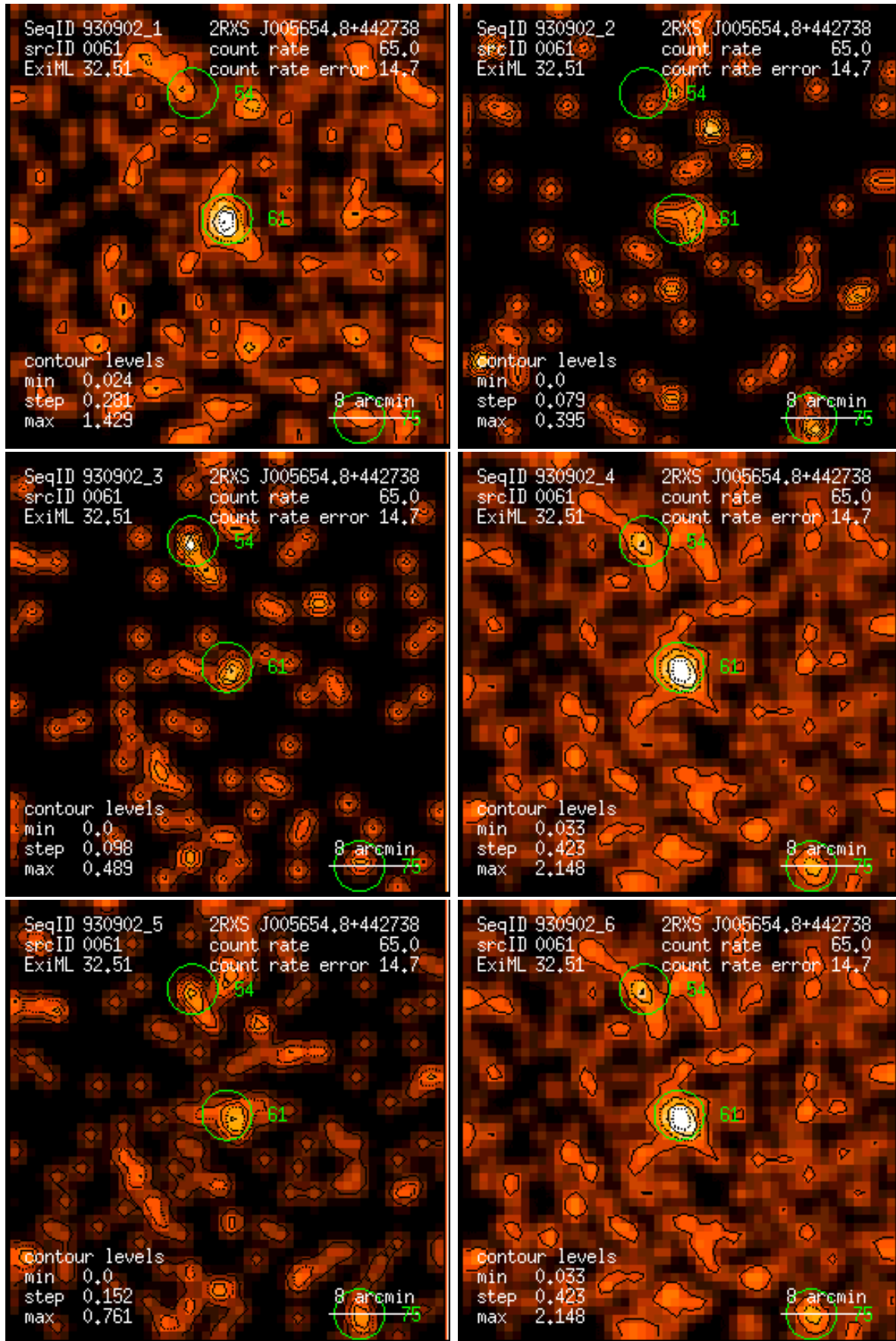
Figure 61: RASS 930902: detection 0061: band rate images, Gaussian filter: (1) PSPC channels 11 – 41, (2) 52 – 90, (3) 91 – 201, (4) 11 – 235, (5) 52 – 201, (6) 11 – 201. Broad band rates in counts/ks. Band rate contour levels in counts/ks/arcmin 2 .
