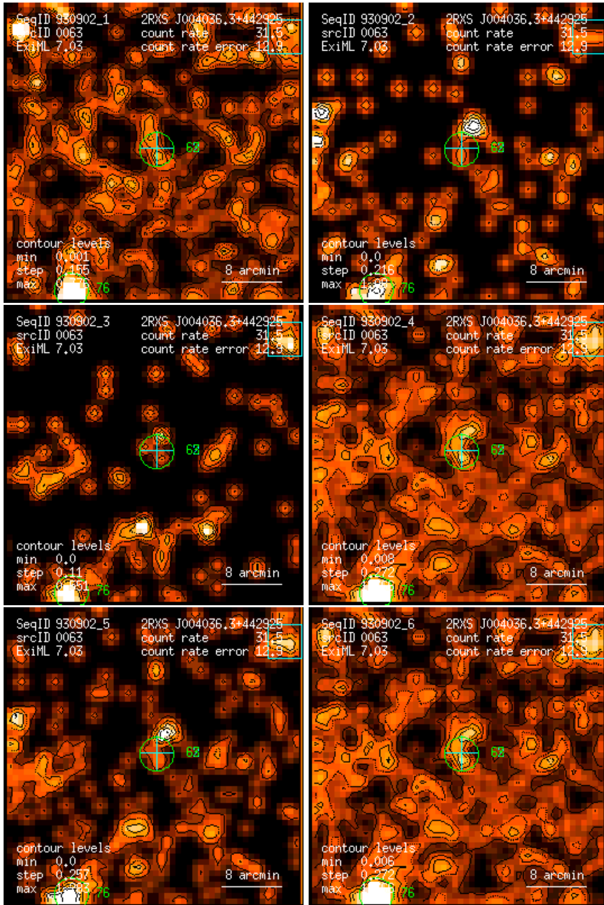
Figure 63: RASS 930902: detection 0063: band rate images, Gaussian filter: (1) PSPC channels 11 – 41, (2) 52 – 90, (3) 91 – 201, (4) 11 – 235, (5) 52 – 201, (6) 11 – 201. Broad band rates in counts/ks. Band rate contour levels in counts/ks/arcmin 2 .
