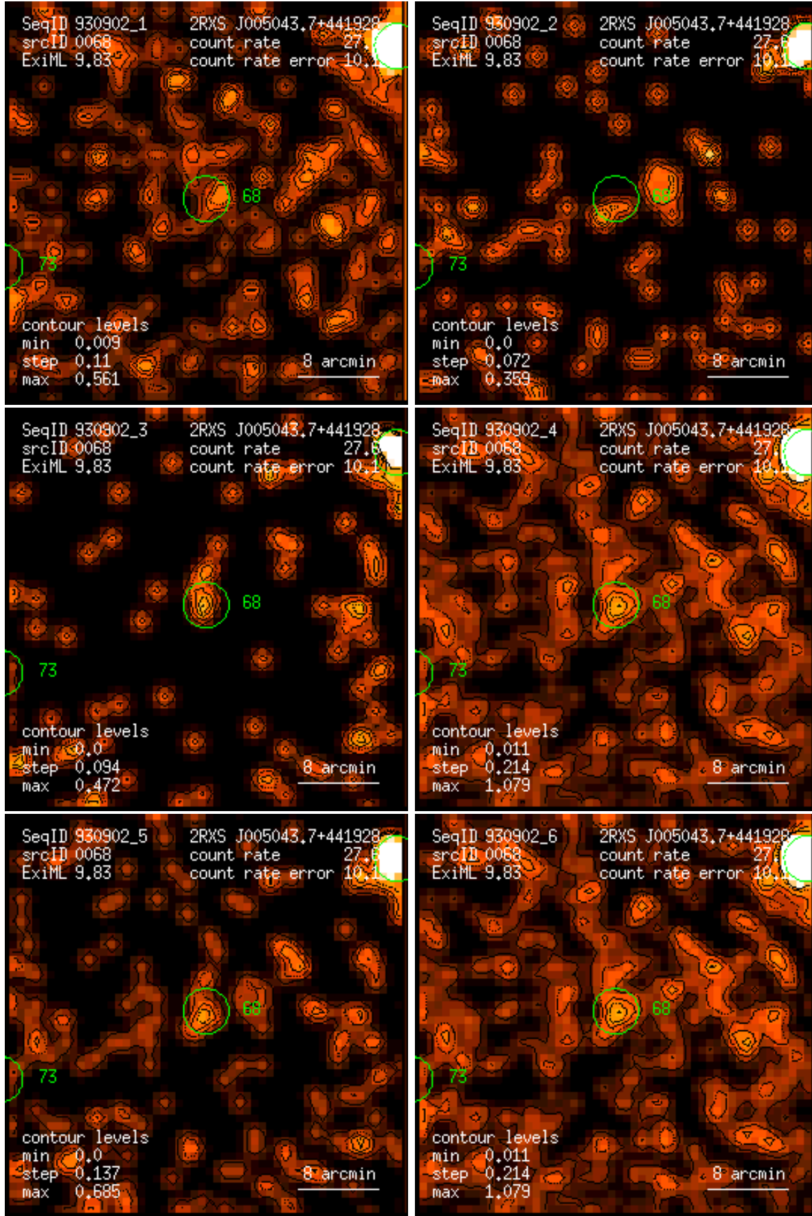
Figure 68: RASS 930902: detection 0068: band rate images, Gaussian filter: (1) PSPC channels 11 – 41, (2) 52 – 90, (3) 91 – 201, (4) 11 – 235, (5) 52 – 201, (6) 11 – 201. Broad band rates in counts/ks. Band rate contour levels in counts/ks/arcmin 2 .
