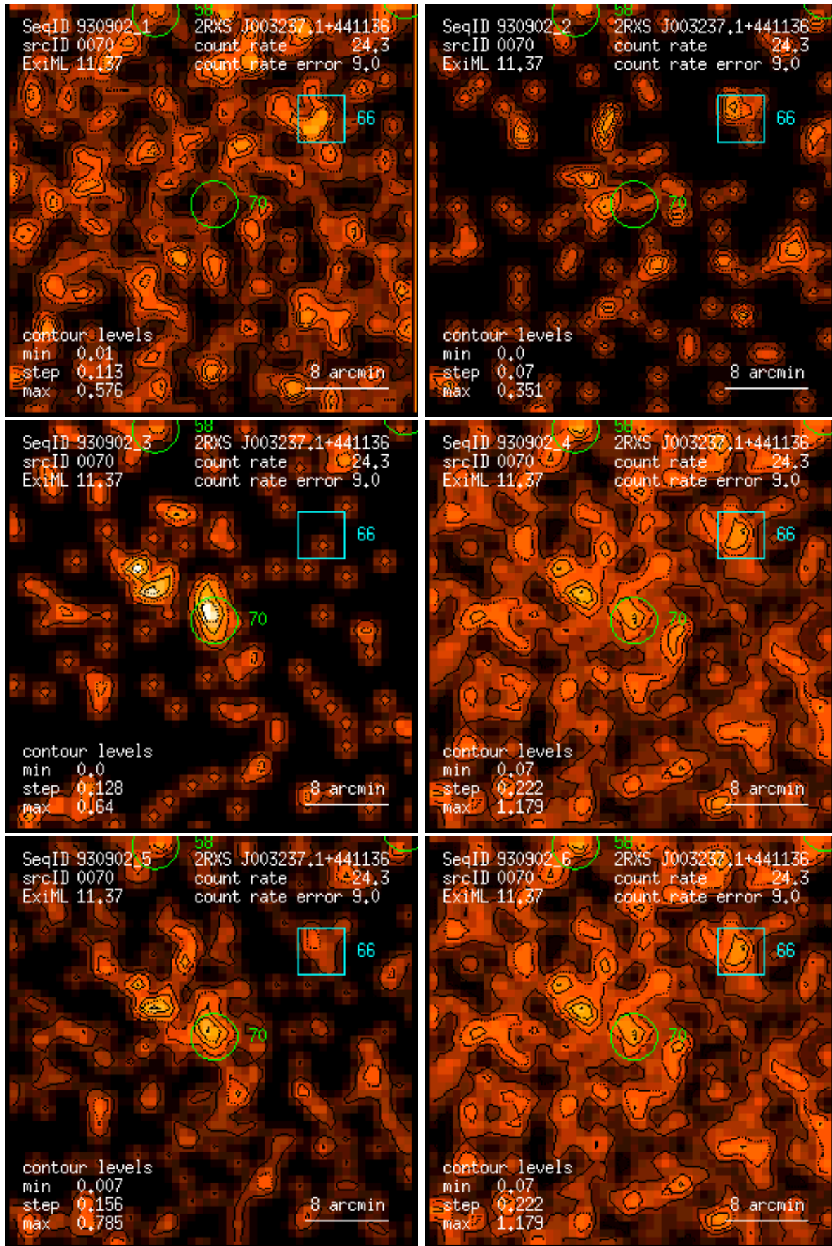
Figure 70: RASS 930902: detection 0070: band rate images, Gaussian filter: (1) PSPC channels 11 – 41, (2) 52 – 90, (3) 91 – 201, (4) 11 – 235, (5) 52 – 201, (6) 11 – 201. Broad band rates in counts/ks. Band rate contour levels in counts/ks/arcmin 2 .
