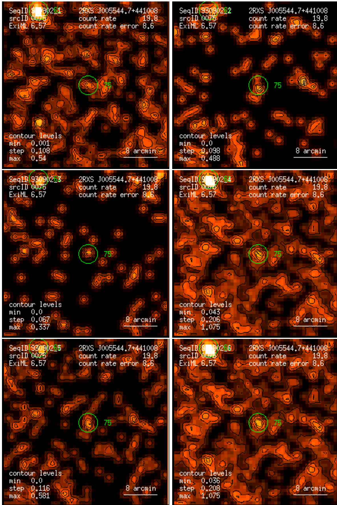
Figure 75: RASS 930902: detection 0075: band rate images, Gaussian filter: (1) PSPC channels 11 – 41, (2) 52 – 90, (3) 91 – 201, (4) 11 – 235, (5) 52 – 201, (6) 11 – 201. Broad band rates in counts/ks. Band rate contour levels in counts/ks/arcmin 2 .
