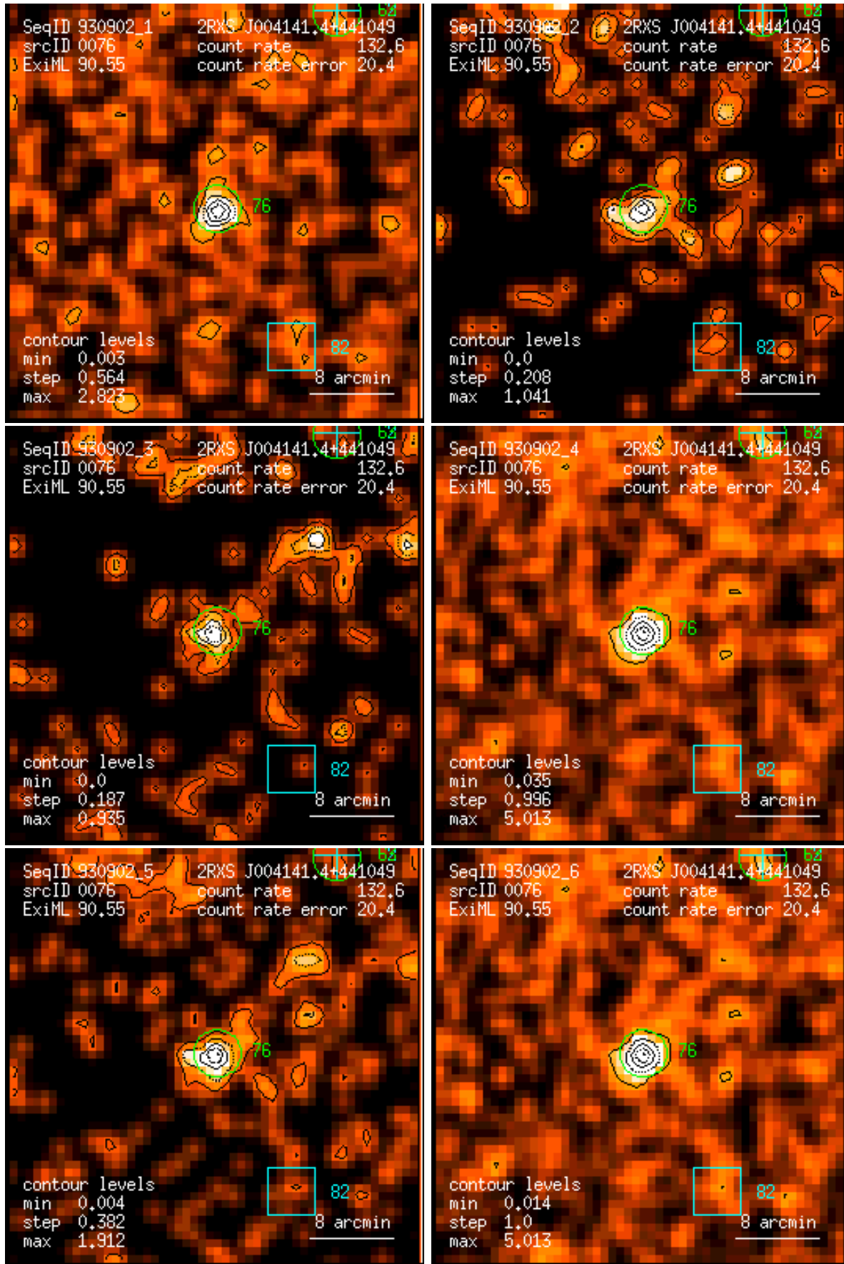
Figure 76: RASS 930902: detection 0076: band rate images, Gaussian filter: (1) PSPC channels 11 – 41, (2) 52 – 90, (3) 91 – 201, (4) 11 – 235, (5) 52 – 201, (6) 11 – 201. Broad band rates in counts/ks. Band rate contour levels in counts/ks/arcmin 2 .
