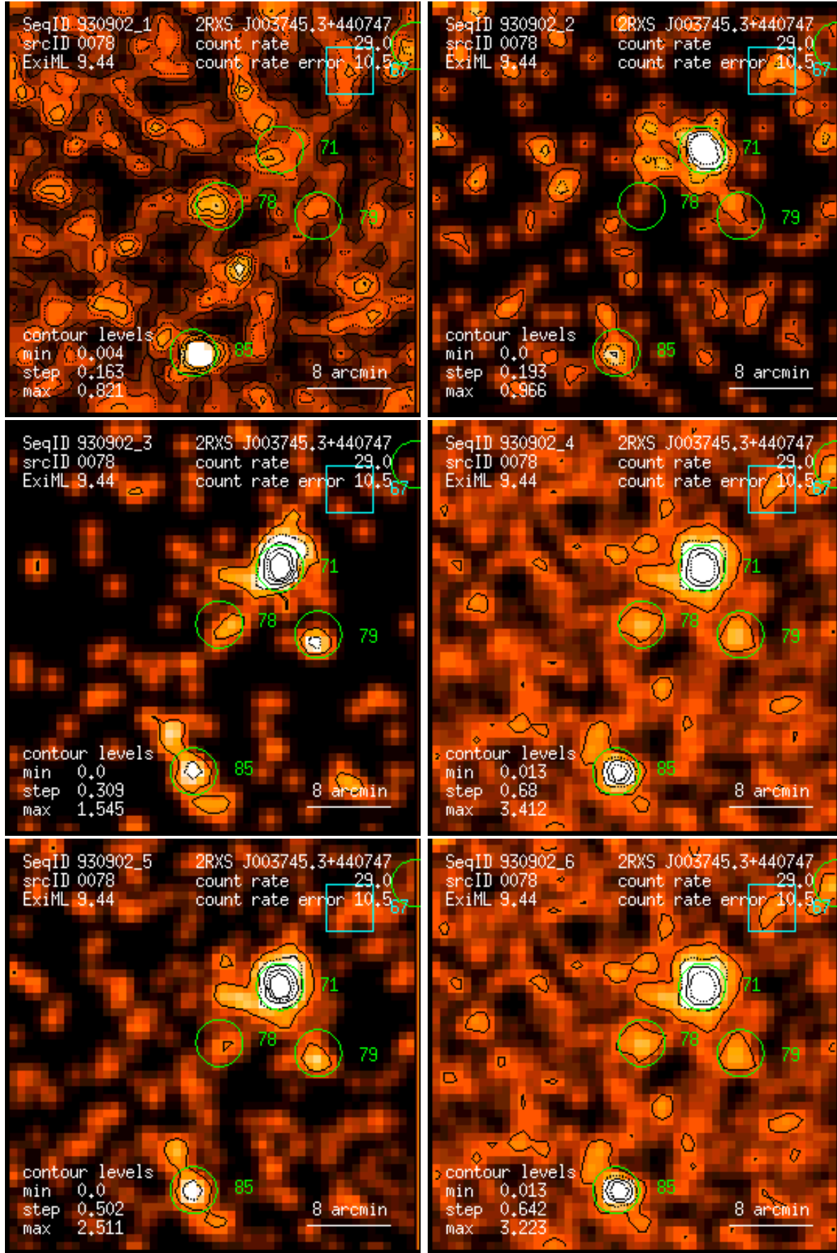
Figure 78: RASS 930902: detection 0078: band rate images, Gaussian filter: (1) PSPC channels 11 – 41, (2) 52 – 90, (3) 91 – 201, (4) 11 – 235, (5) 52 – 201, (6) 11 – 201. Broad band rates in counts/ks. Band rate contour levels in counts/ks/arcmin 2 .
