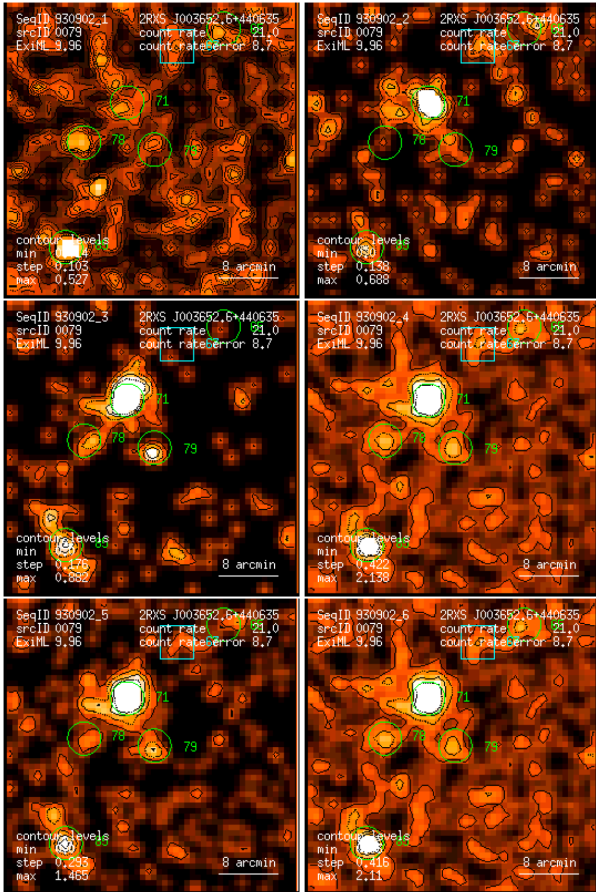
Figure 79: RASS 930902: detection 0079: band rate images, Gaussian filter: (1) PSPC channels 11 – 41, (2) 52 – 90, (3) 91 – 201, (4) 11 – 235, (5) 52 – 201, (6) 11 – 201. Broad band rates in counts/ks. Band rate contour levels in counts/ks/arcmin 2 .
