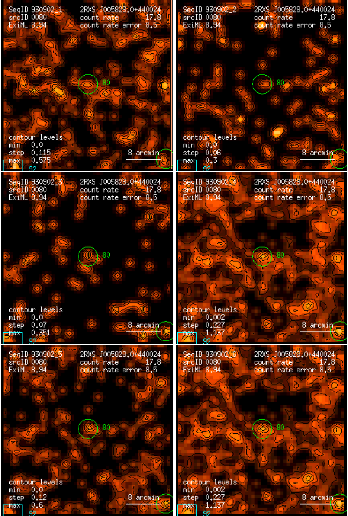
Figure 80: RASS 930902: detection 0080: band rate images, Gaussian filter: (1) PSPC channels 11 – 41, (2) 52 – 90, (3) 91 – 201, (4) 11 – 235, (5) 52 – 201, (6) 11 – 201. Broad band rates in counts/ks. Band rate contour levels in counts/ks/arcmin 2 .
