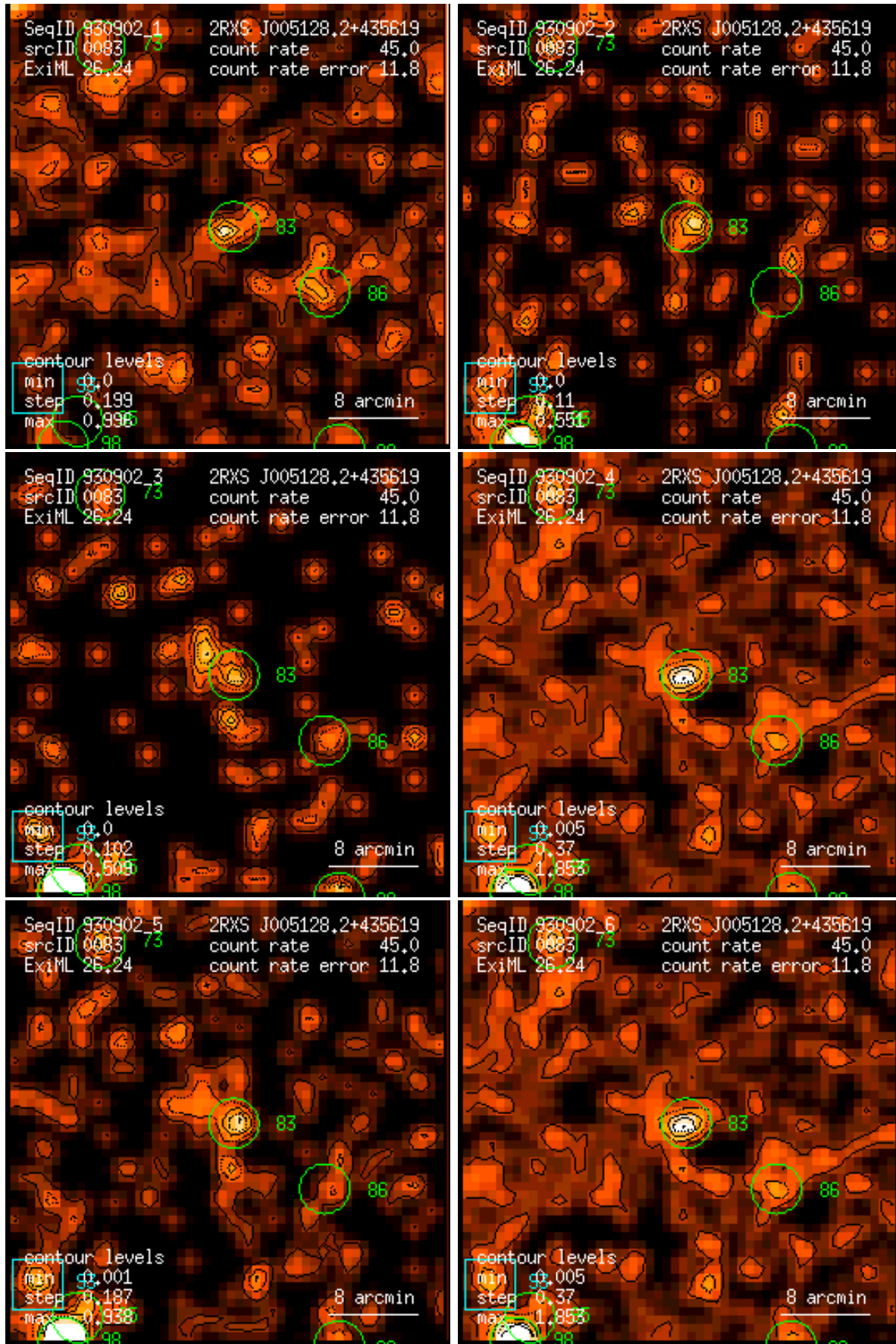
Figure 83: RASS 930902: detection 0083: band rate images, Gaussian filter: (1) PSPC channels 11 – 41, (2) 52 – 90, (3) 91 – 201, (4) 11 – 235, (5) 52 – 201, (6) 11 – 201. Broad band rates in counts/ks. Band rate contour levels in counts/ks/arcmin 2 .
