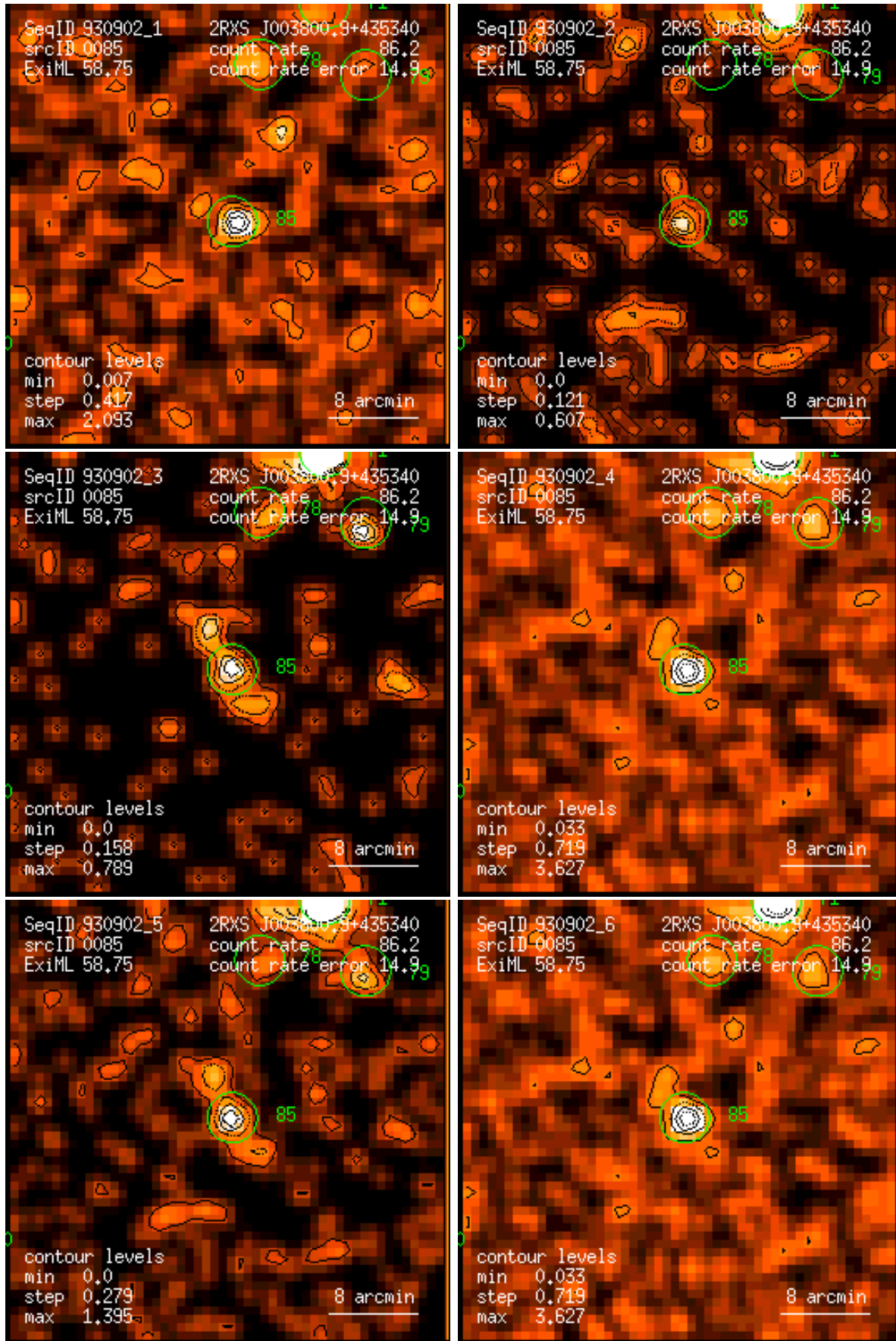
Figure 85: RASS 930902: detection 0085: band rate images, Gaussian filter: (1) PSPC channels 11 – 41, (2) 52 – 90, (3) 91 – 201, (4) 11 – 235, (5) 52 – 201, (6) 11 – 201. Broad band rates in counts/ks. Band rate contour levels in counts/ks/arcmin 2 .
