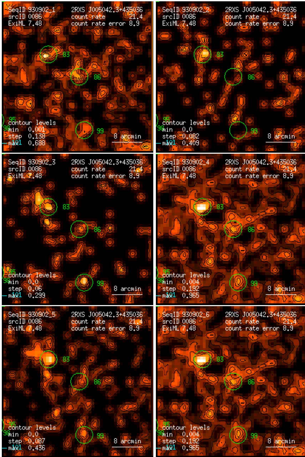
Figure 86: RASS 930902: detection 0086: band rate images, Gaussian filter: (1) PSPC channels 11 – 41, (2) 52 – 90, (3) 91 – 201, (4) 11 – 235, (5) 52 – 201, (6) 11 – 201. Broad band rates in counts/ks. Band rate contour levels in counts/ks/arcmin 2 .
