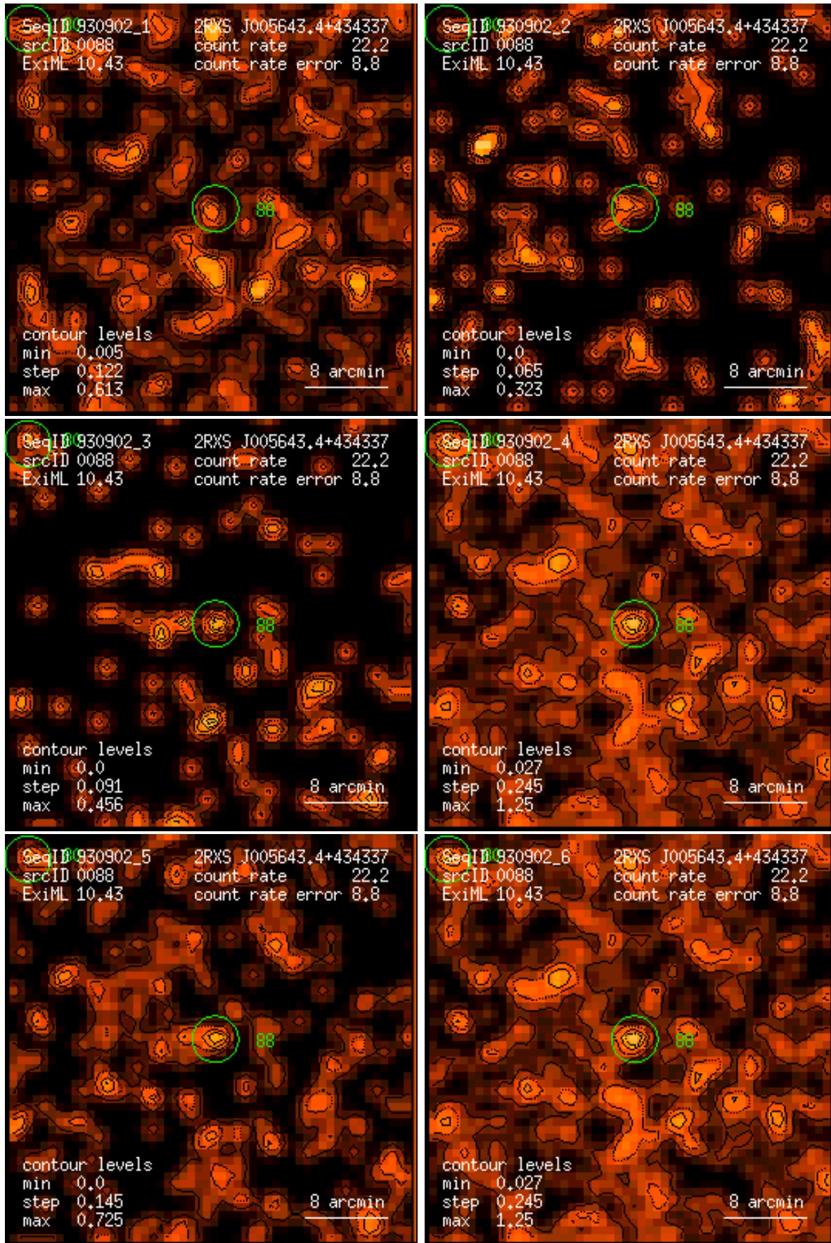
Figure 88: RASS 930902: detection 0088: band rate images, Gaussian filter: (1) PSPC channels 11 – 41, (2) 52 – 90, (3) 91 – 201, (4) 11 – 235, (5) 52 – 201, (6) 11 – 201. Broad band rates in counts/ks. Band rate contour levels in counts/ks/arcmin 2 .
