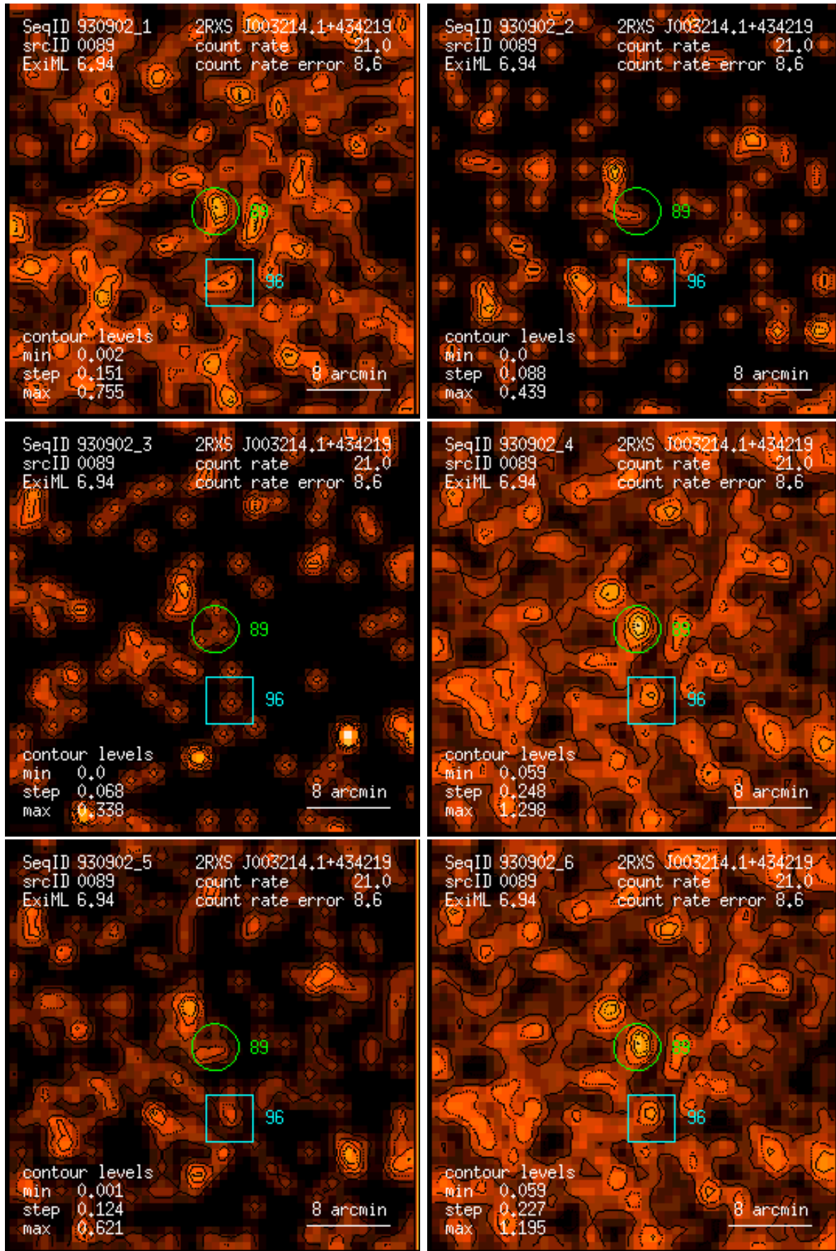
Figure 89: RASS 930902: detection 0089: band rate images, Gaussian filter: (1) PSPC channels 11 – 41, (2) 52 – 90, (3) 91 – 201, (4) 11 – 235, (5) 52 – 201, (6) 11 – 201. Broad band rates in counts/ks. Band rate contour levels in counts/ks/arcmin 2 .
