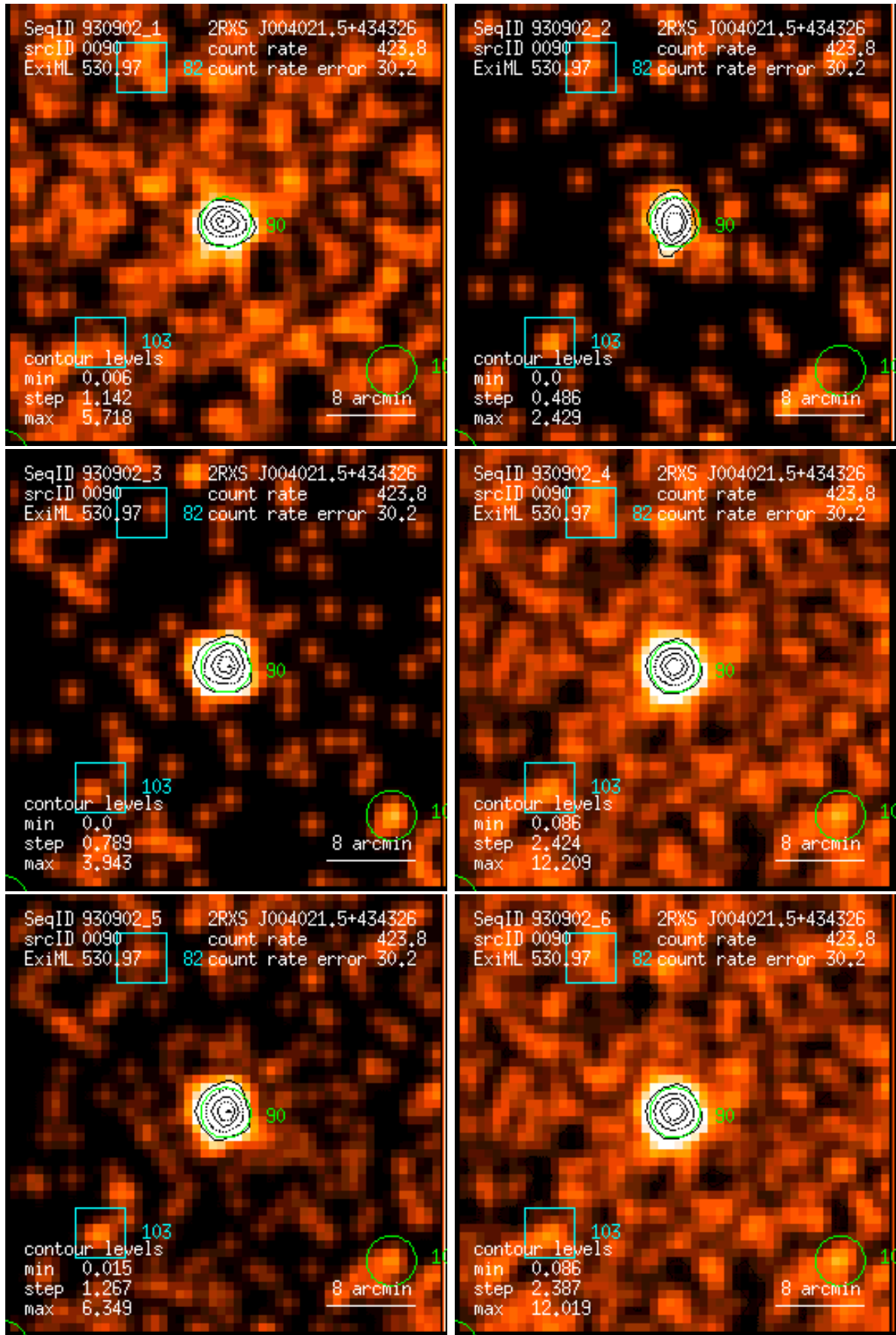
Figure 90: RASS 930902: detection 0090: band rate images, Gaussian filter: (1) PSPC channels 11 – 41, (2) 52 – 90, (3) 91 – 201, (4) 11 – 235, (5) 52 – 201, (6) 11 – 201. Broad band rates in counts/ks. Band rate contour levels in counts/ks/arcmin 2 .
