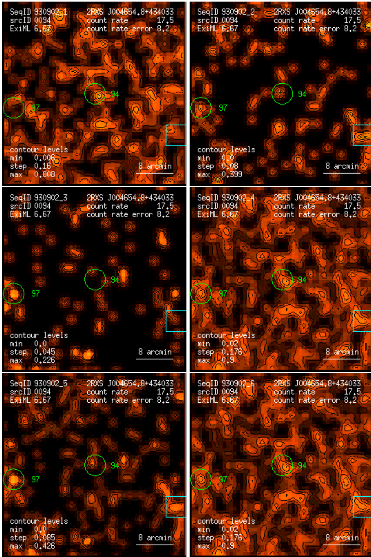
Figure 94: RASS 930902: detection 0094: band rate images, Gaussian filter: (1) PSPC channels 11 – 41, (2) 52 – 90, (3) 91 – 201, (4) 11 – 235, (5) 52 – 201, (6) 11 – 201. Broad band rates in counts/ks. Band rate contour levels in counts/ks/arcmin 2 .
