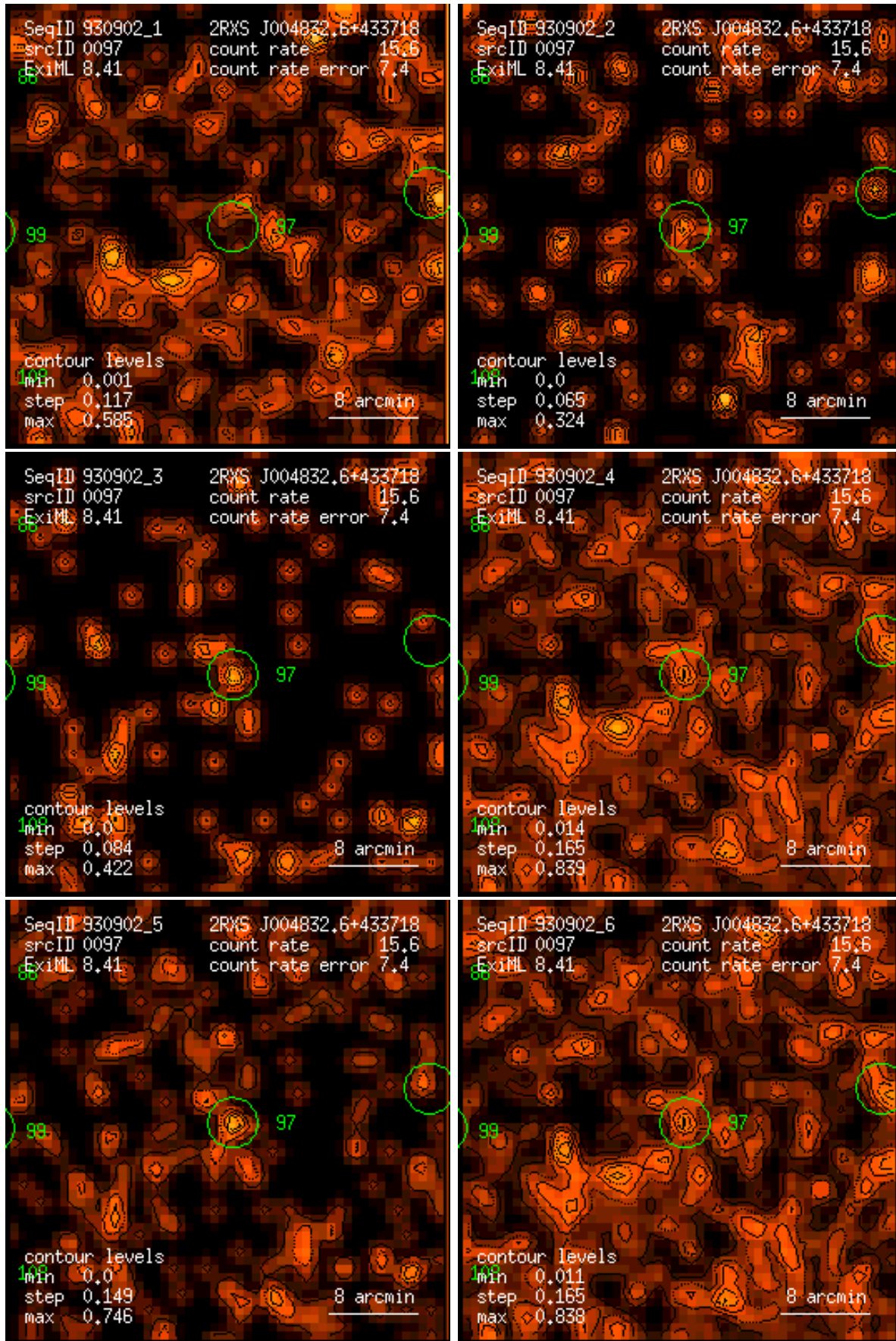
Figure 97: RASS 930902: detection 0097: band rate images, Gaussian filter: (1) PSPC channels 11 – 41, (2) 52 – 90, (3) 91 – 201, (4) 11 – 235, (5) 52 – 201, (6) 11 – 201. Broad band rates in counts/ks. Band rate contour levels in counts/ks/arcmin 2 .
