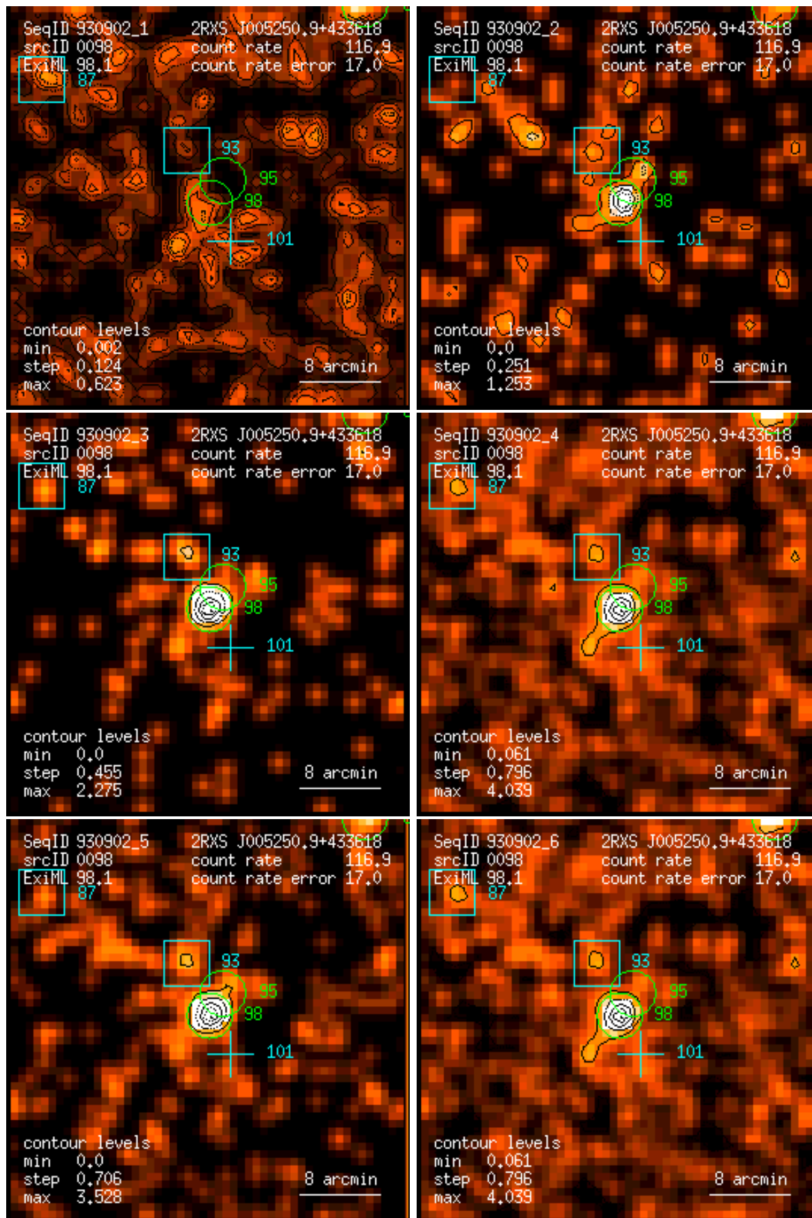
Figure 98: RASS 930902: detection 0098: band rate images, Gaussian filter: (1) PSPC channels 11 – 41, (2) 52 – 90, (3) 91 – 201, (4) 11 – 235, (5) 52 – 201, (6) 11 – 201. Broad band rates in counts/ks. Band rate contour levels in counts/ks/arcmin 2 .
