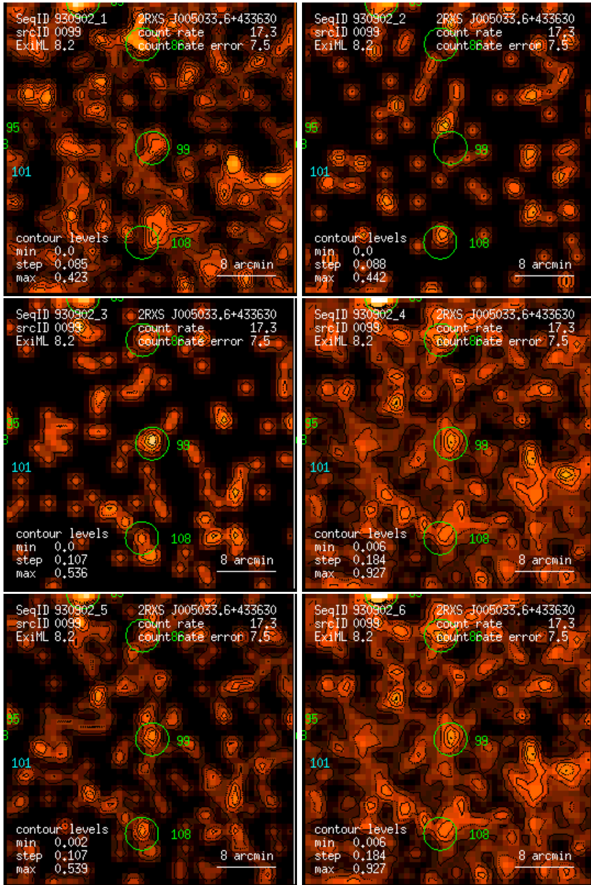
Figure 99: RASS 930902: detection 0099: band rate images, Gaussian filter: (1) PSPC channels 11 – 41, (2) 52 – 90, (3) 91 – 201, (4) 11 – 235, (5) 52 – 201, (6) 11 – 201. Broad band rates in counts/ks. Band rate contour levels in counts/ks/arcmin 2 .
