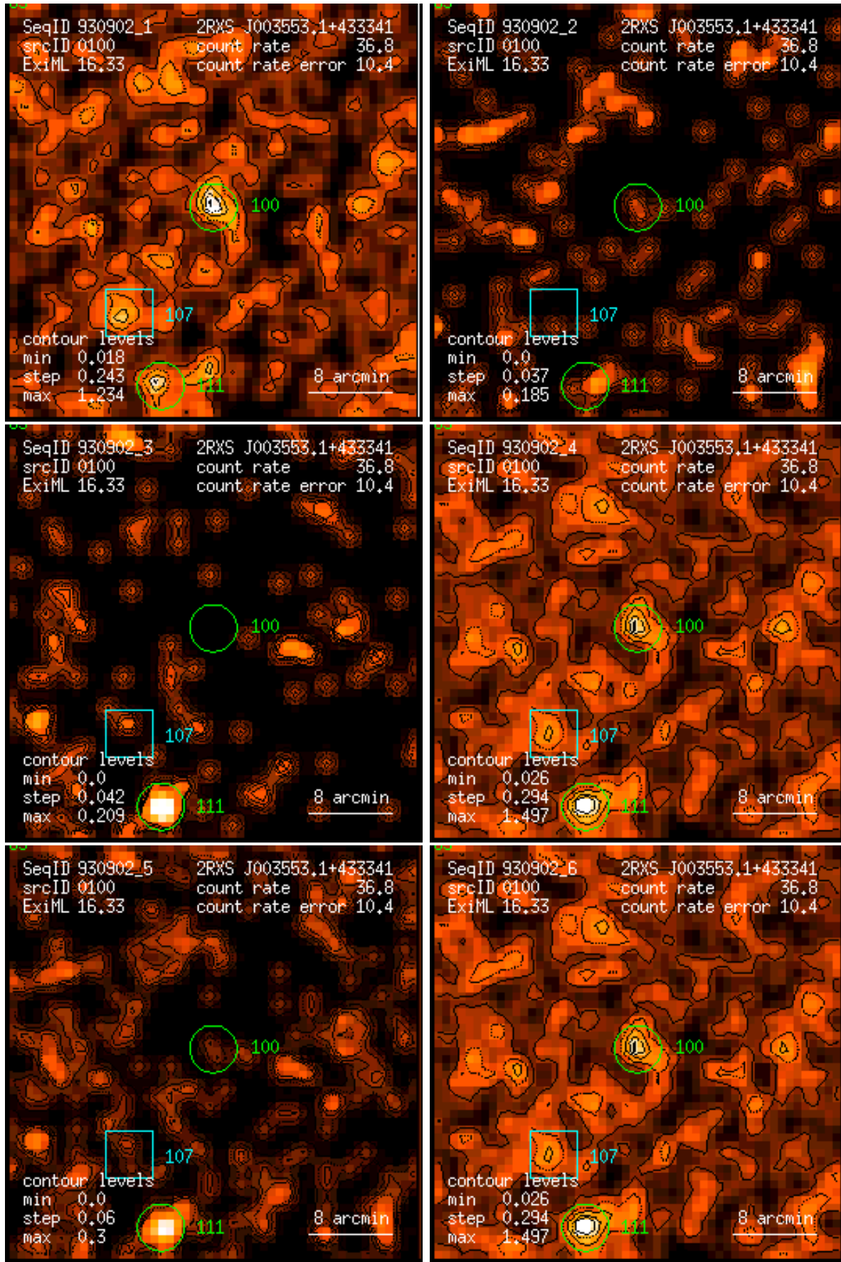
Figure 100: RASS 930902: detection 0100: band rate images, Gaussian filter: (1) PSPC channels 11 – 41, (2) 52 – 90, (3) 91 – 201, (4) 11 – 235, (5) 52 – 201, (6) 11 – 201. Broad band rates in counts/ks. Band rate contour levels in counts/ks/arcmin 2 .
