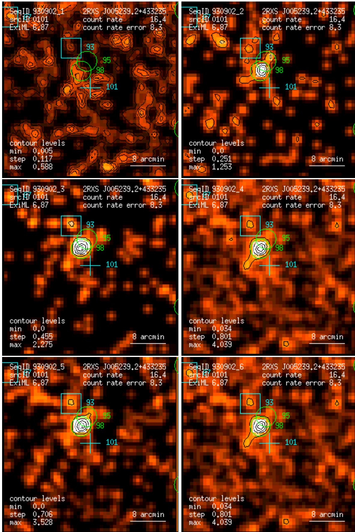
Figure 101: RASS 930902: detection 0101: band rate images, Gaussian filter: (1) PSPC channels 11 – 41, (2) 52 – 90, (3) 91 – 201, (4) 11 – 235, (5) 52 – 201, (6) 11 – 201. Broad band rates in counts/ks. Band rate contour levels in counts/ks/arcmin 2 .
