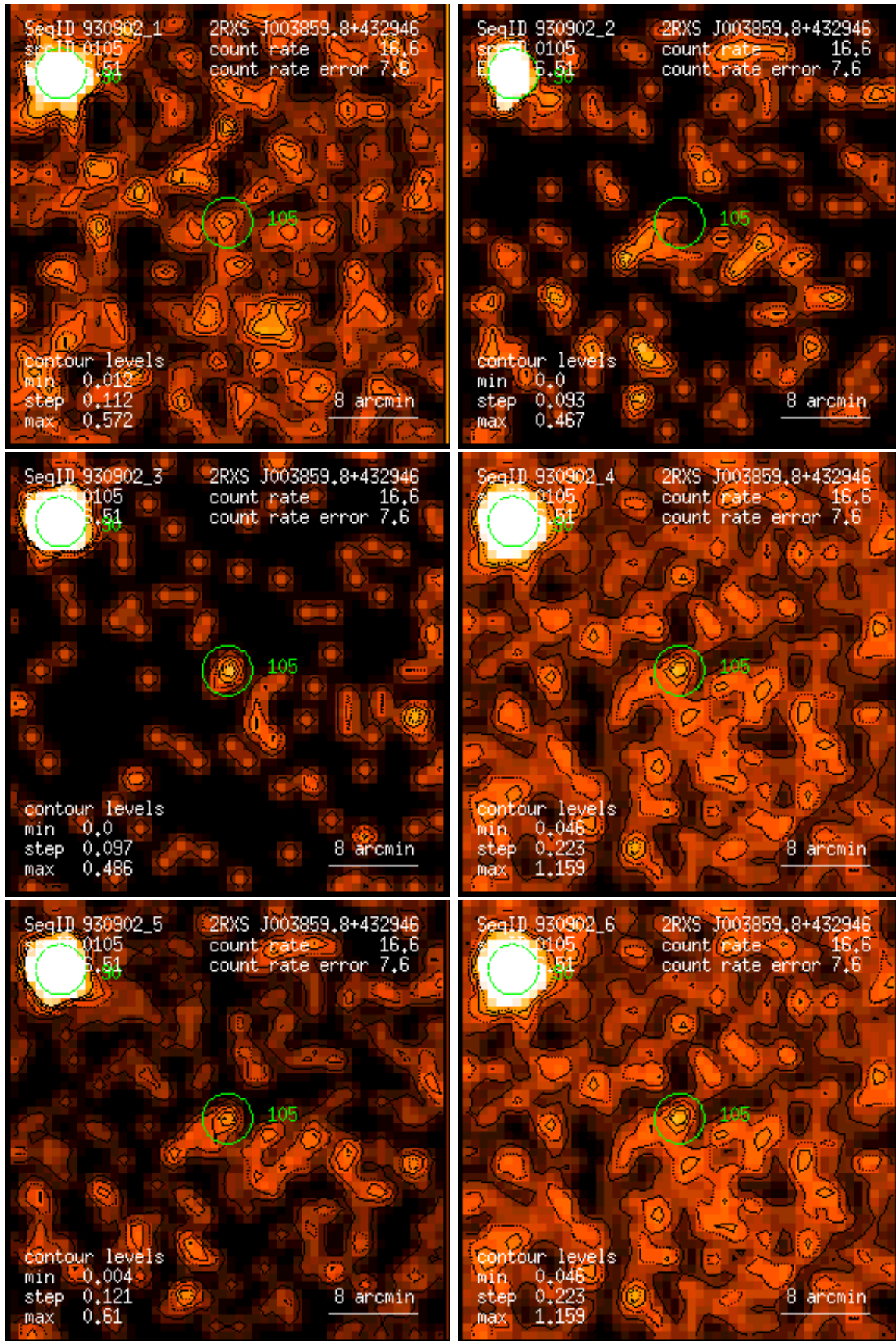
Figure 105: RASS 930902: detection 0105: band rate images, Gaussian filter: (1) PSPC channels 11 – 41, (2) 52 – 90, (3) 91 – 201, (4) 11 – 235, (5) 52 – 201, (6) 11 – 201. Broad band rates in counts/ks. Band rate contour levels in counts/ks/arcmin 2 .
