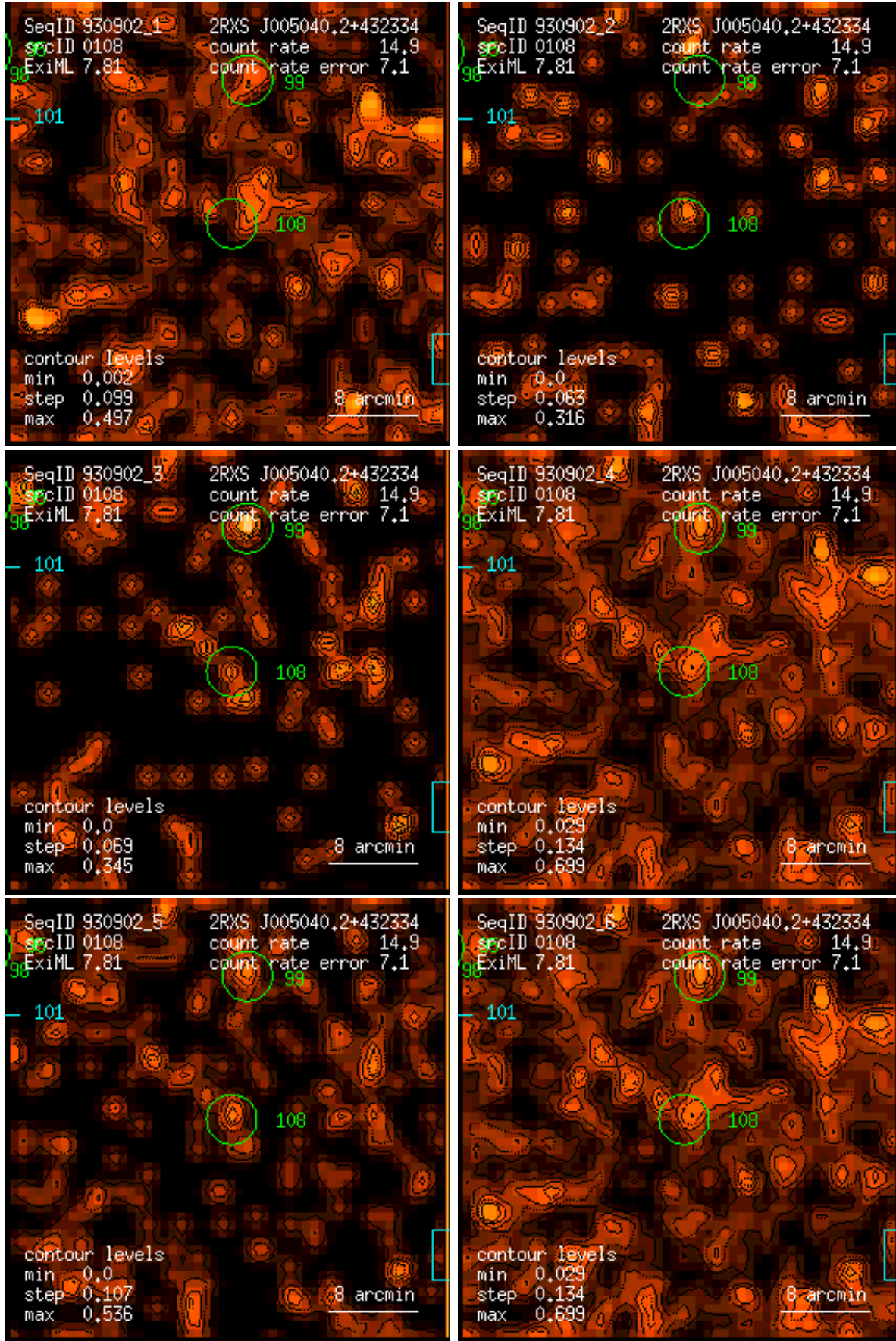
Figure 108: RASS 930902: detection 0108: band rate images, Gaussian filter: (1) PSPC channels 11 – 41, (2) 52 – 90, (3) 91 – 201, (4) 11 – 235, (5) 52 – 201, (6) 11 – 201. Broad band rates in counts/ks. Band rate contour levels in counts/ks/arcmin 2 .
