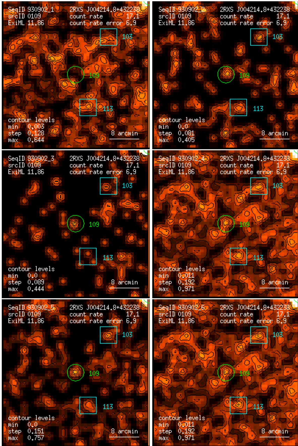
Figure 109: RASS 930902: detection 0109: band rate images, Gaussian filter: (1) PSPC channels 11 – 41, (2) 52 – 90, (3) 91 – 201, (4) 11 – 235, (5) 52 – 201, (6) 11 – 201. Broad band rates in counts/ks. Band rate contour levels in counts/ks/arcmin 2 .
