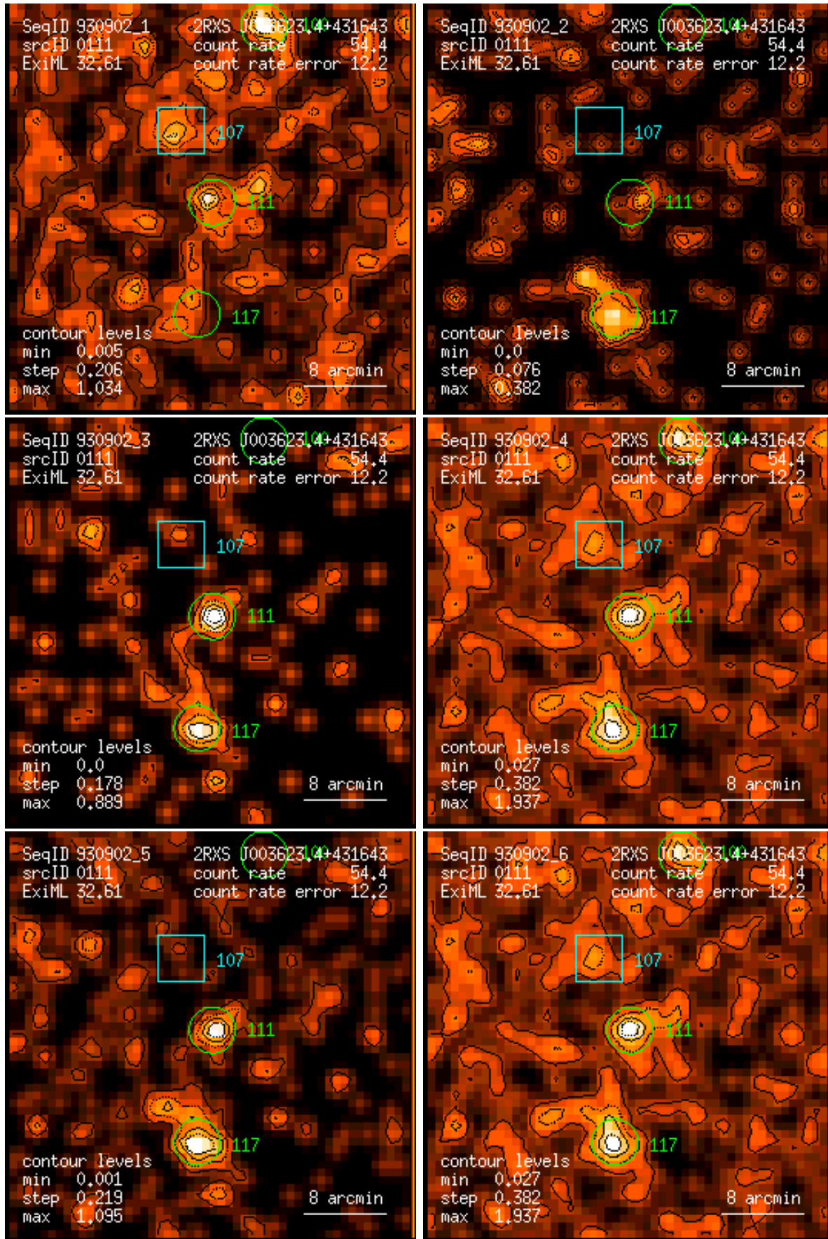
Figure 111: RASS 930902: detection 0111: band rate images, Gaussian filter: (1) PSPC channels 11 – 41, (2) 52 – 90, (3) 91 – 201, (4) 11 – 235, (5) 52 – 201, (6) 11 – 201. Broad band rates in counts/ks. Band rate contour levels in counts/ks/arcmin 2 .
