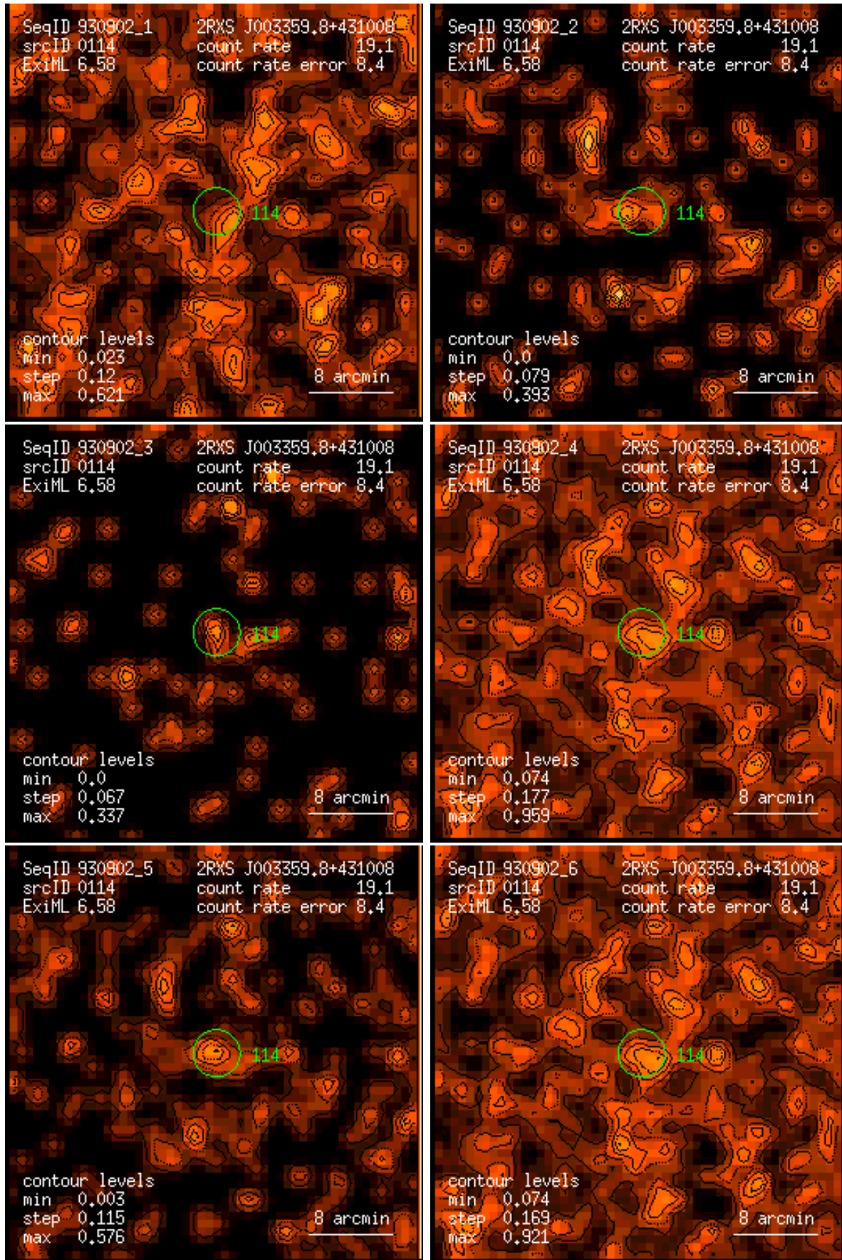
Figure 114: RASS 930902: detection 0114: band rate images, Gaussian filter: (1) PSPC channels 11 – 41, (2) 52 – 90, (3) 91 – 201, (4) 11 – 235, (5) 52 – 201, (6) 11 – 201. Broad band rates in counts/ks. Band rate contour levels in counts/ks/arcmin 2 .
