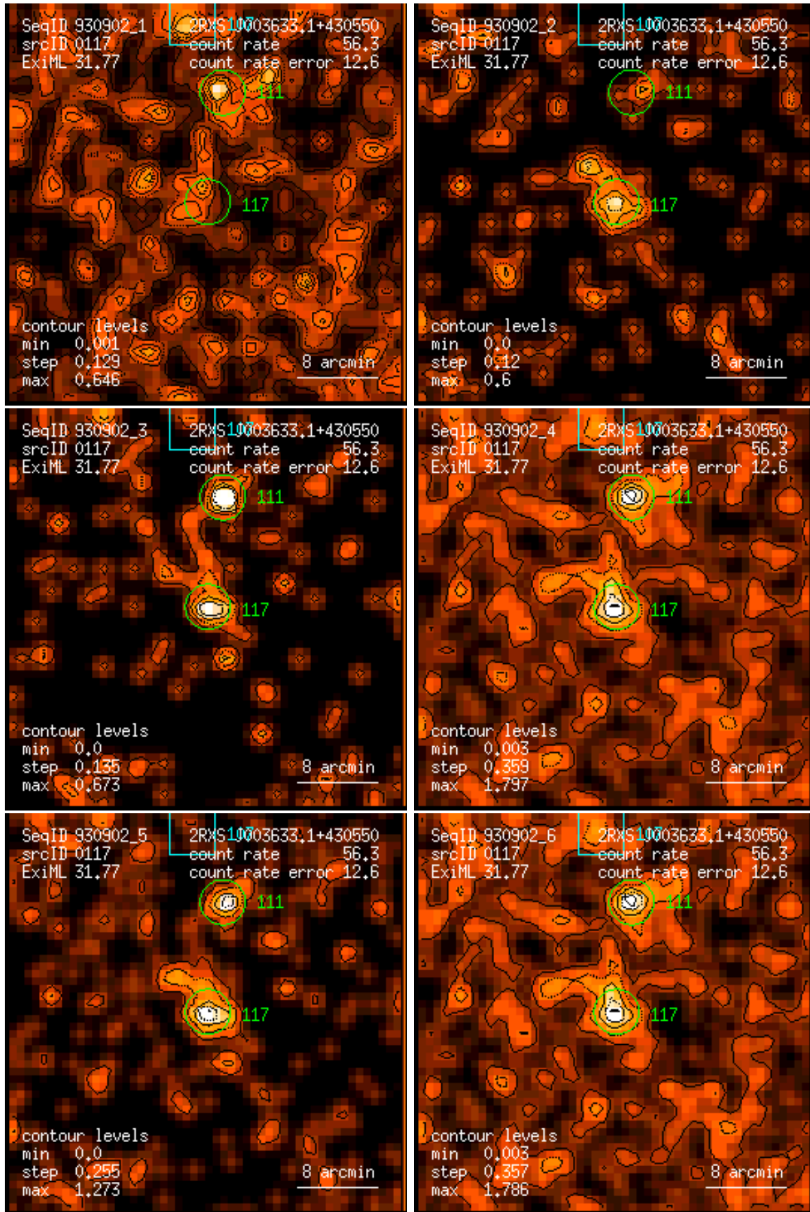
Figure 117: RASS 930902: detection 0117: band rate images, Gaussian filter: (1) PSPC channels 11 – 41, (2) 52 – 90, (3) 91 – 201, (4) 11 – 235, (5) 52 – 201, (6) 11 – 201. Broad band rates in counts/ks. Band rate contour levels in counts/ks/arcmin 2 .
