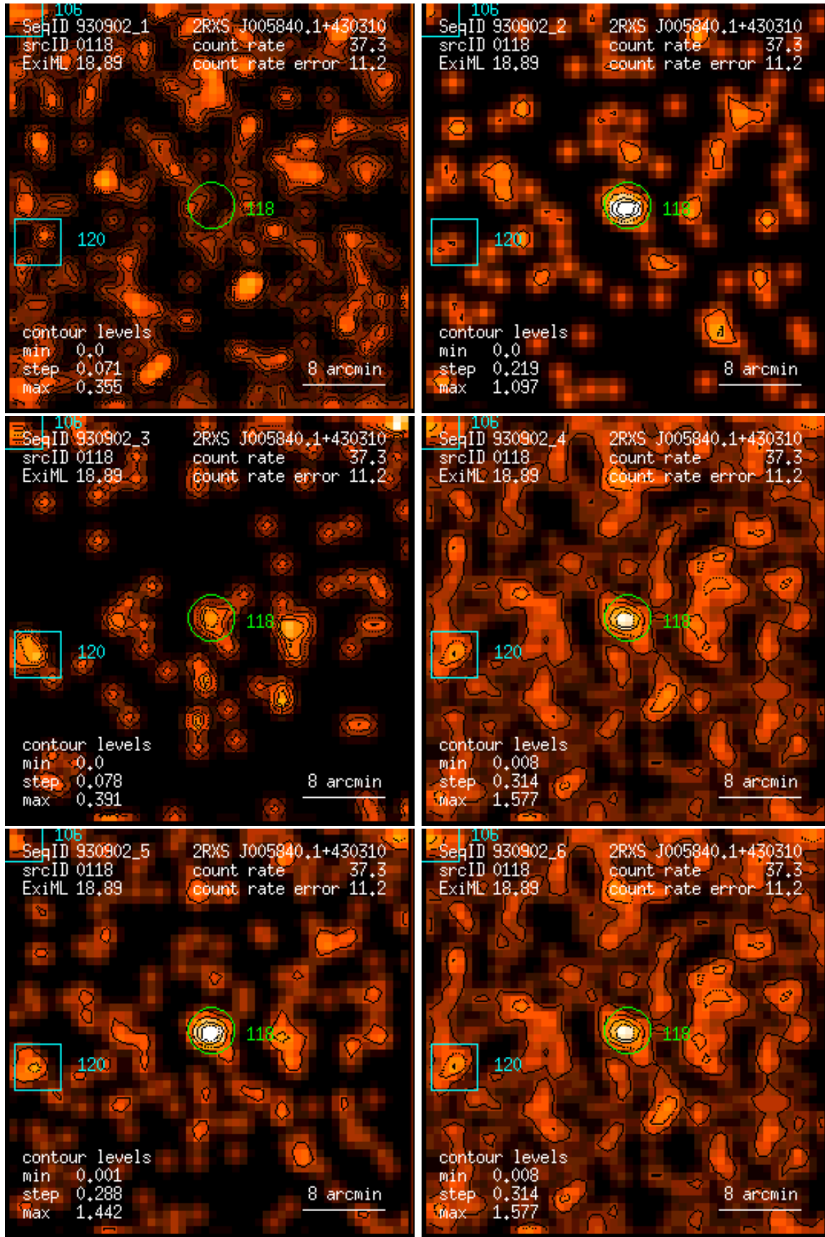
Figure 118: RASS 930902: detection 0118: band rate images, Gaussian filter: (1) PSPC channels 11 – 41, (2) 52 – 90, (3) 91 – 201, (4) 11 – 235, (5) 52 – 201, (6) 11 – 201. Broad band rates in counts/ks. Band rate contour levels in counts/ks/arcmin 2 .
