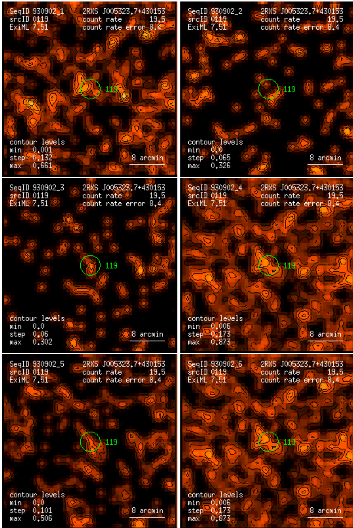
Figure 119: RASS 930902: detection 0119: band rate images, Gaussian filter: (1) PSPC channels 11 – 41, (2) 52 – 90, (3) 91 – 201, (4) 11 – 235, (5) 52 – 201, (6) 11 – 201. Broad band rates in counts/ks. Band rate contour levels in counts/ks/arcmin 2 .
