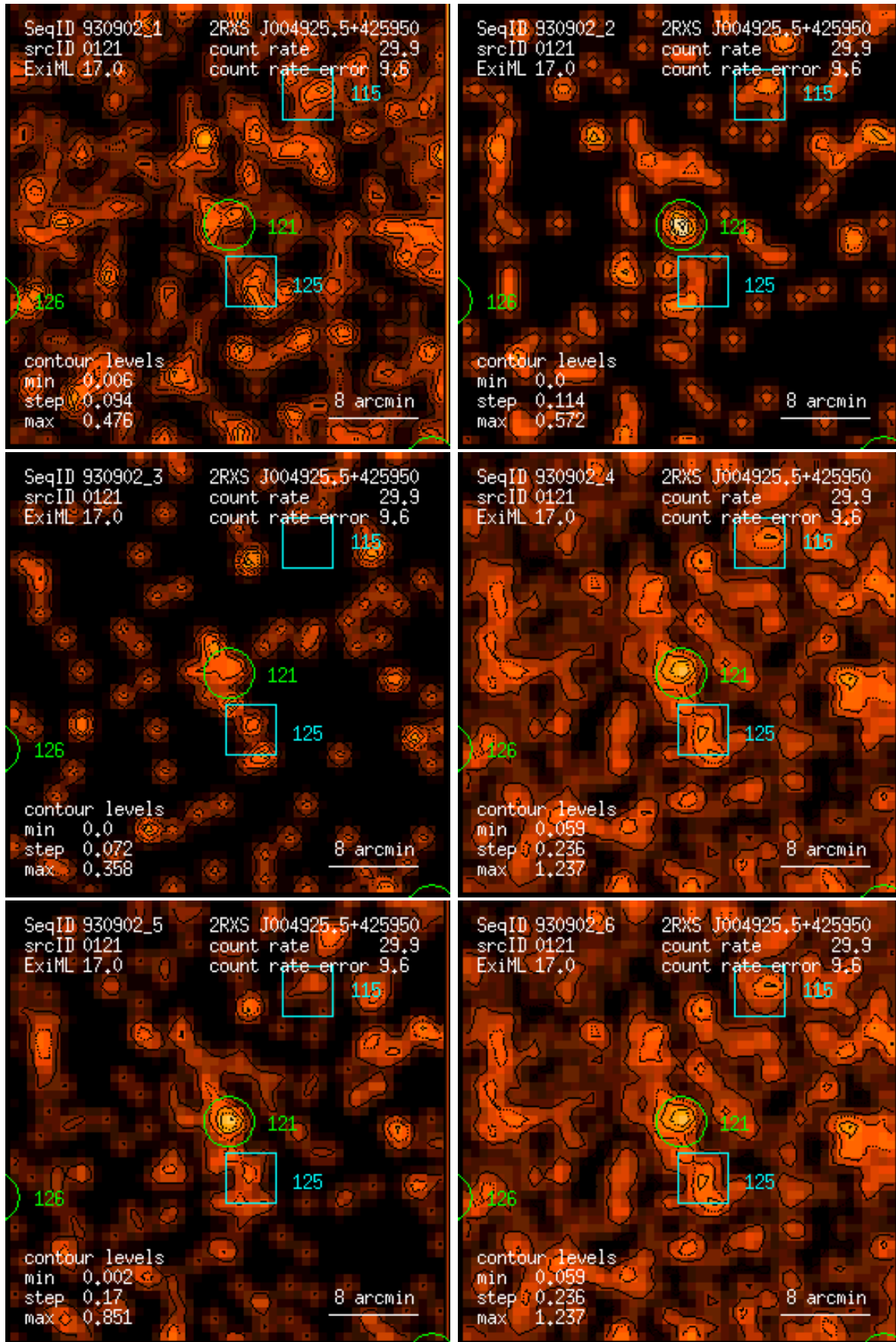
Figure 121: RASS 930902: detection 0121: band rate images, Gaussian filter: (1) PSPC channels 11 – 41, (2) 52 – 90, (3) 91 – 201, (4) 11 – 235, (5) 52 – 201, (6) 11 – 201. Broad band rates in counts/ks. Band rate contour levels in counts/ks/arcmin 2 .
