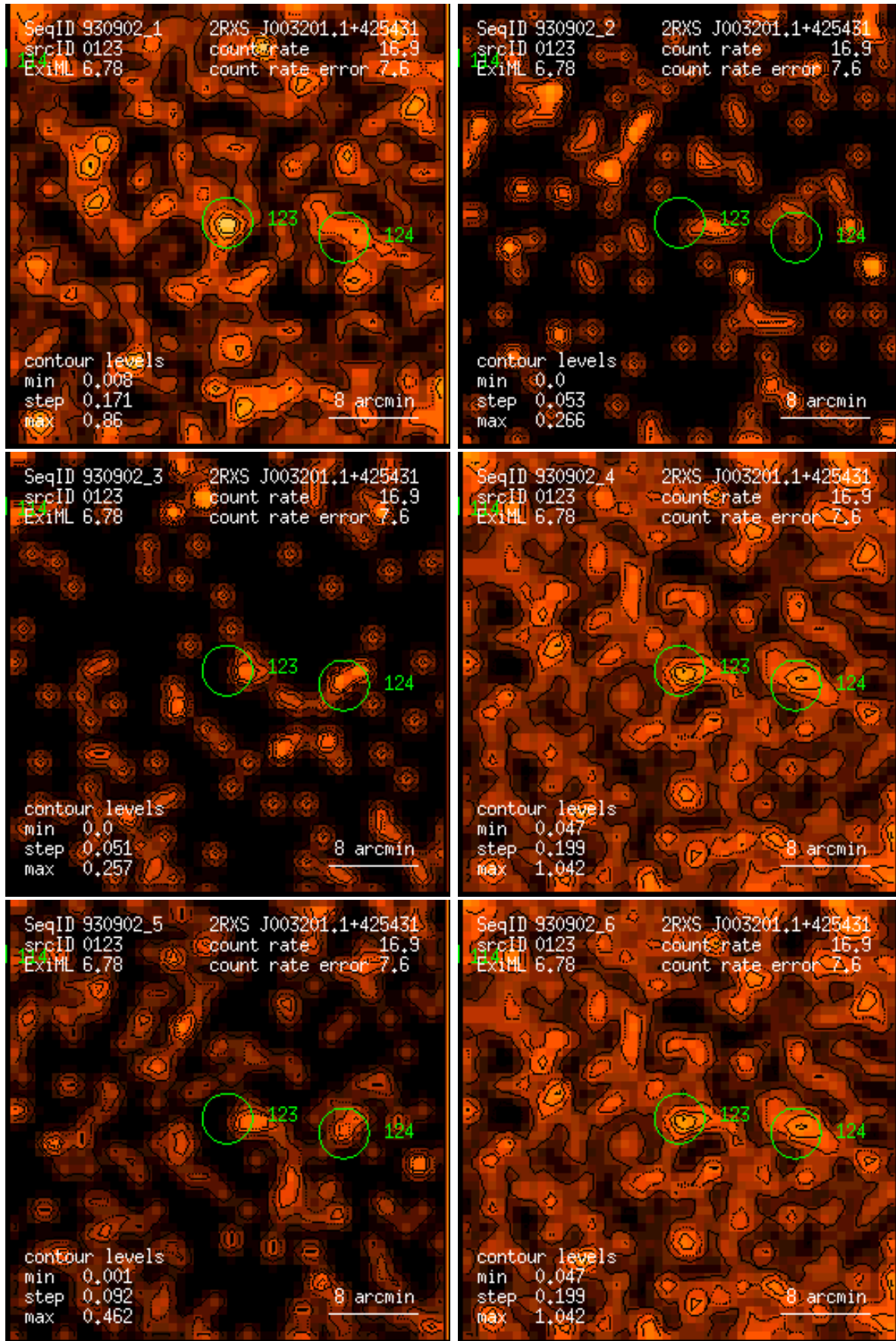
Figure 123: RASS 930902: detection 0123: band rate images, Gaussian filter: (1) PSPC channels 11 – 41, (2) 52 – 90, (3) 91 – 201, (4) 11 – 235, (5) 52 – 201, (6) 11 – 201. Broad band rates in counts/ks. Band rate contour levels in counts/ks/arcmin 2 .
