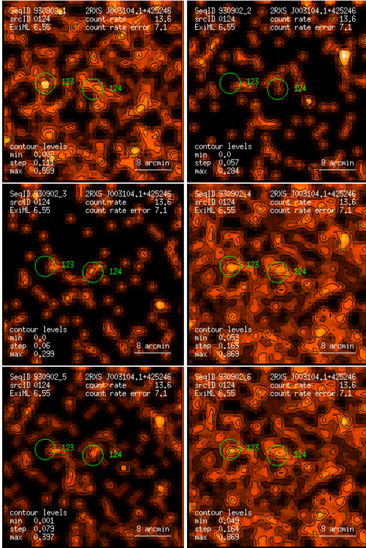
Figure 124: RASS 930902: detection 0124: band rate images, Gaussian filter: (1) PSPC channels 11 – 41, (2) 52 – 90, (3) 91 – 201, (4) 11 – 235, (5) 52 – 201, (6) 11 – 201. Broad band rates in counts/ks. Band rate contour levels in counts/ks/arcmin 2 .
