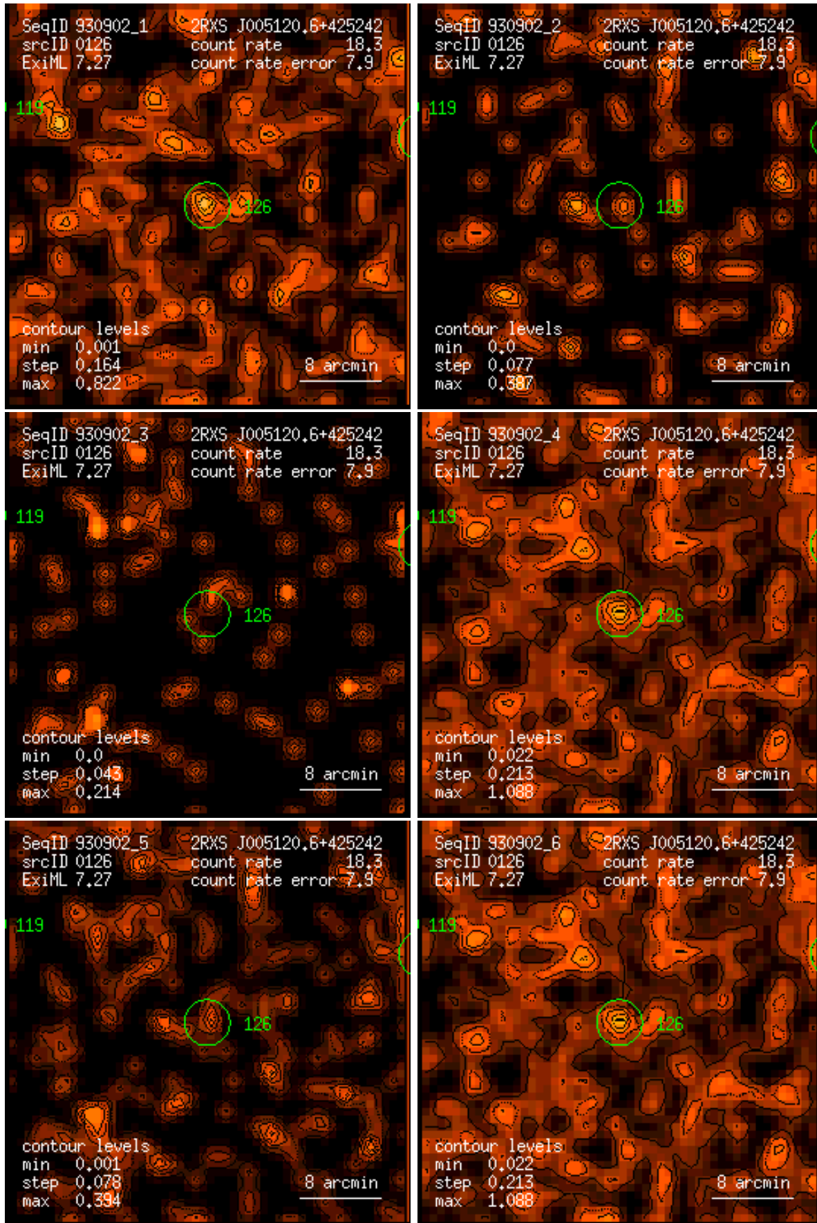
Figure 126: RASS 930902: detection 0126: band rate images, Gaussian filter: (1) PSPC channels 11 – 41, (2) 52 – 90, (3) 91 – 201, (4) 11 – 235, (5) 52 – 201, (6) 11 – 201. Broad band rates in counts/ks. Band rate contour levels in counts/ks/arcmin 2 .
